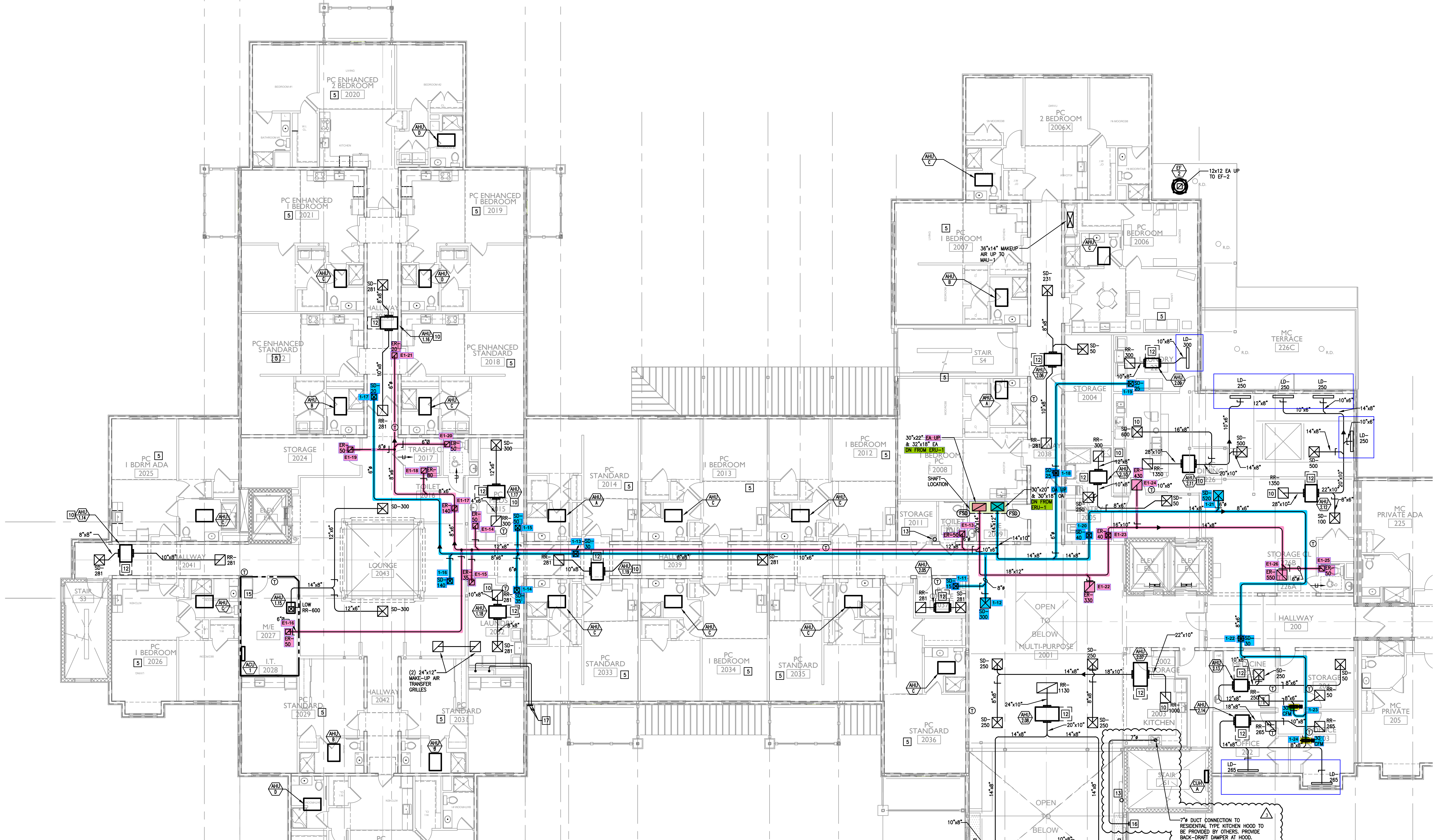
PARTIAL SECOND FLOOR PLAN - MECHANICAL SCALE: 1/8"=1'-0"
