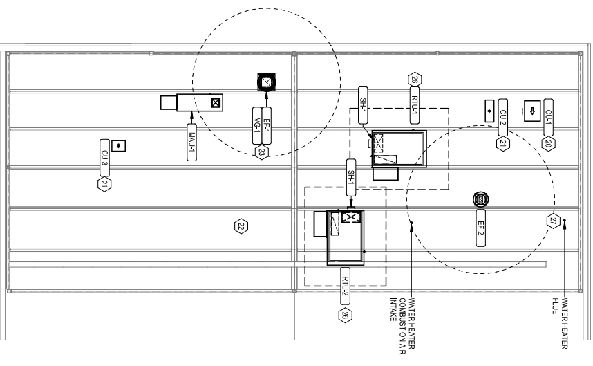
2 ROOF MECHANICAL PLAN 1/8" = 1'-0"
