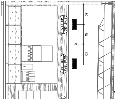
5 HVAC DINING ROOM SECTION 1/4" = 1'-0"
