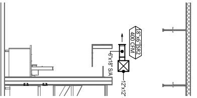
8 HVAC DINING ROOM SECTION 1/4" = 1'-0"
