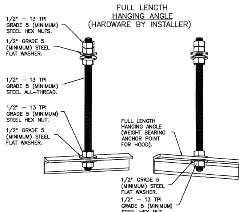
ASSEMBLY INSTRUCTIONS
