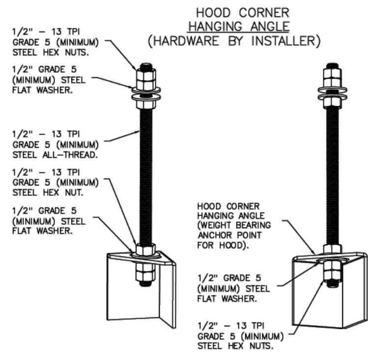
ASSEMBLY INSTRUCTIONS
