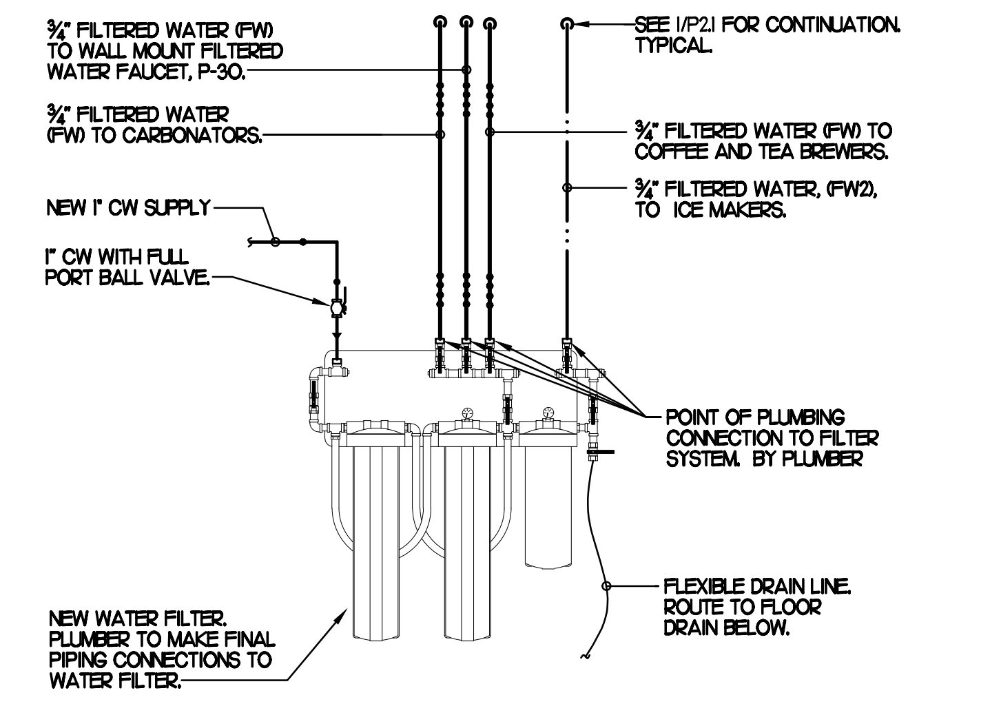
9 WATER FILTER RISER PIPING NO SCALE
