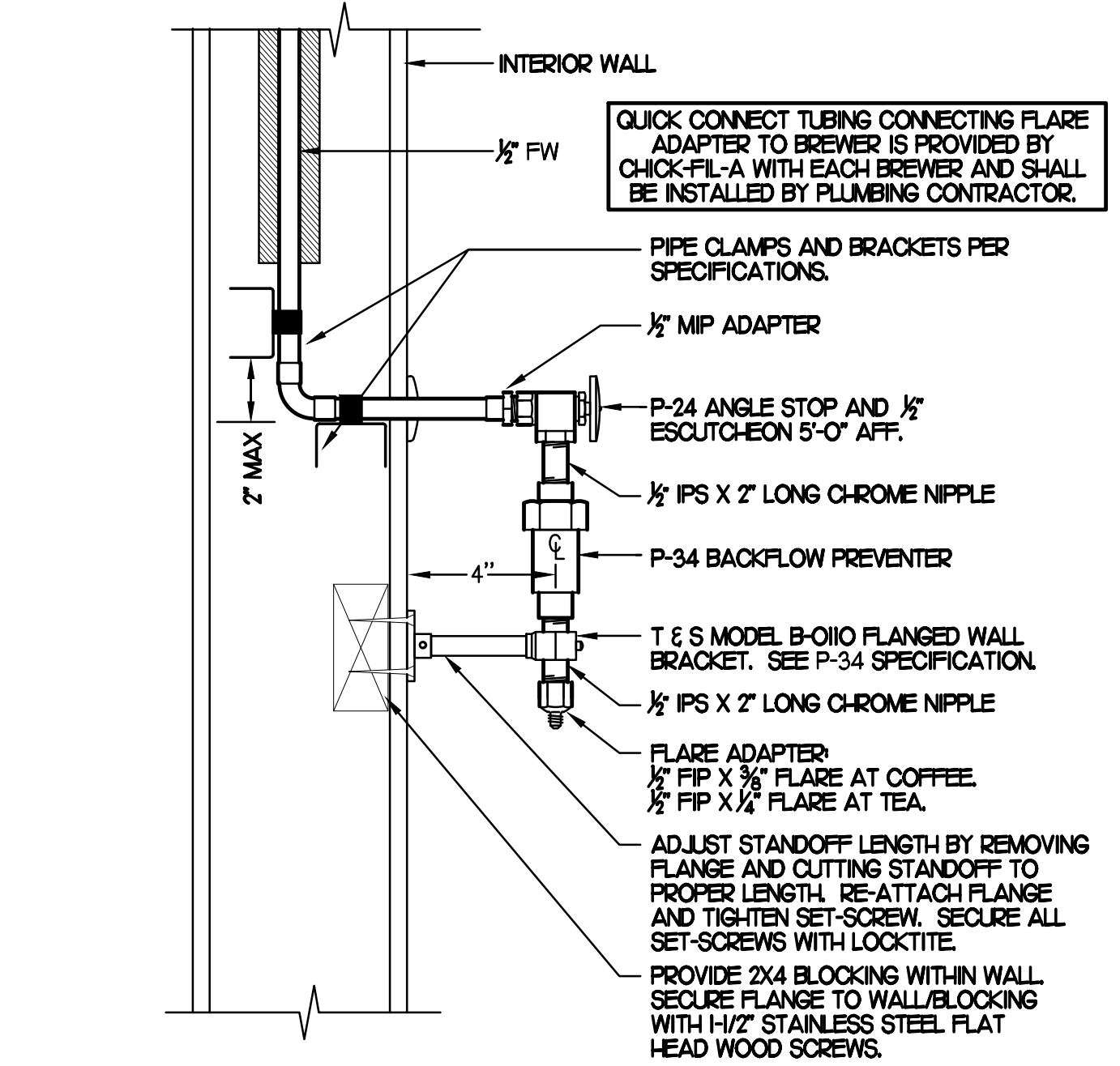
6 COFFEE & TEA BREWER STOP & BFP NO SCALE
