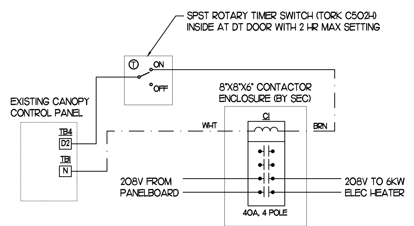
2 OMD ELECTRIC HEATER ADDITION NO SCALE
