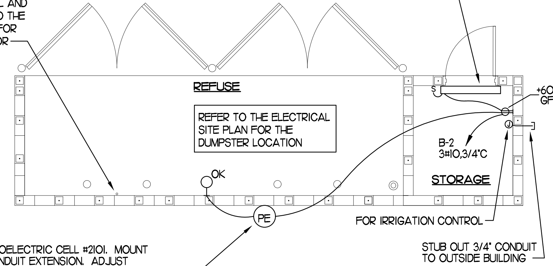
2 REFUSE ENCLOSURE PLAN - ELECTRICAL SCALE: NTS
