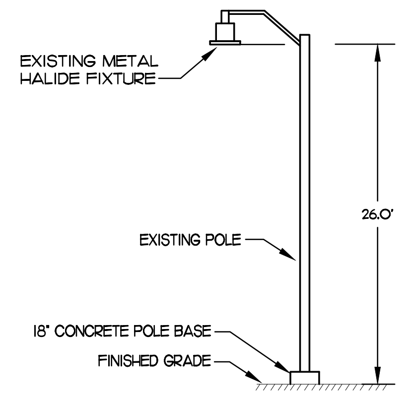
2 SITE LIGHTING POLE DETAIL NOT TO SCALE
