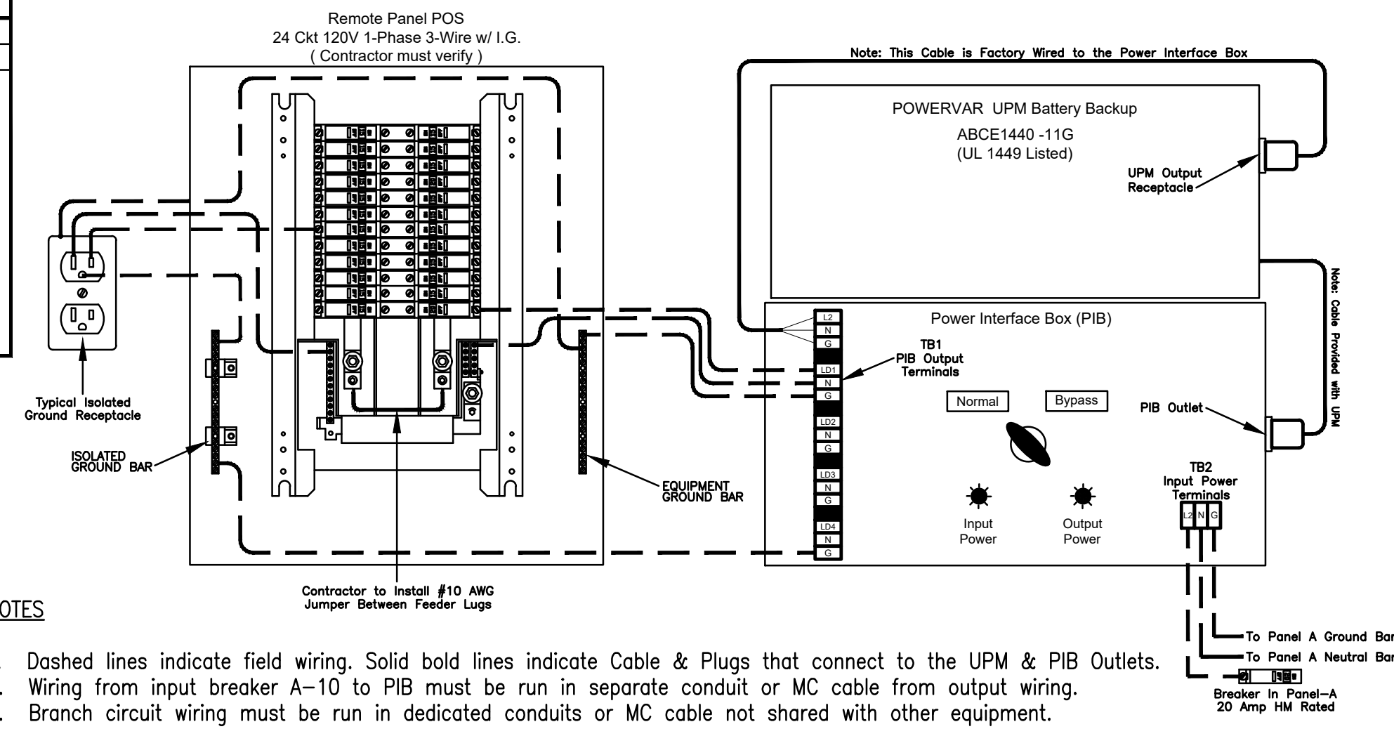
2 POWERVAR LACP with PIB and Panel POS Wiring Diagram NO SCALE
