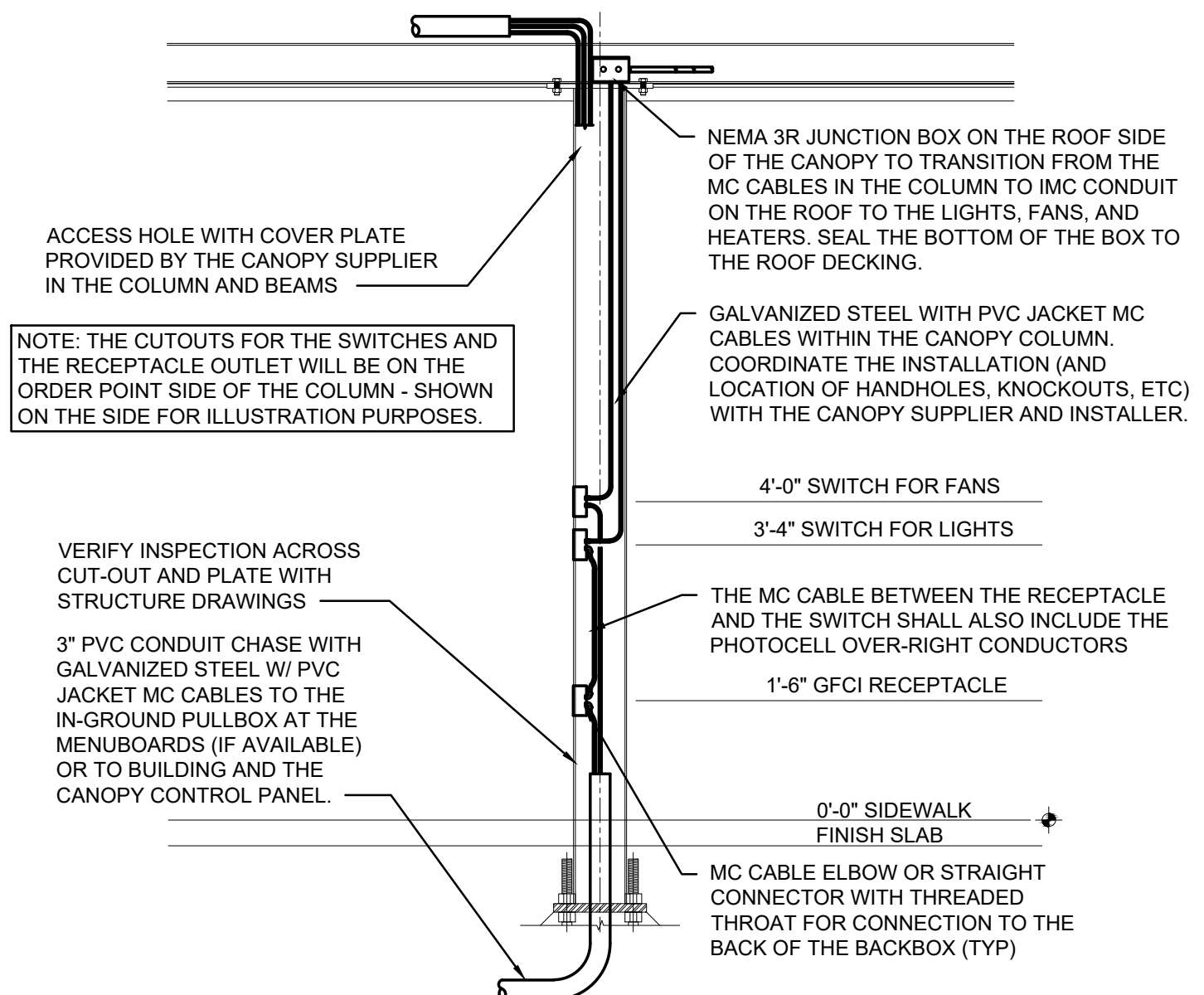
OMD CANOPY COLUMN SECTION NOT TO SCALE
