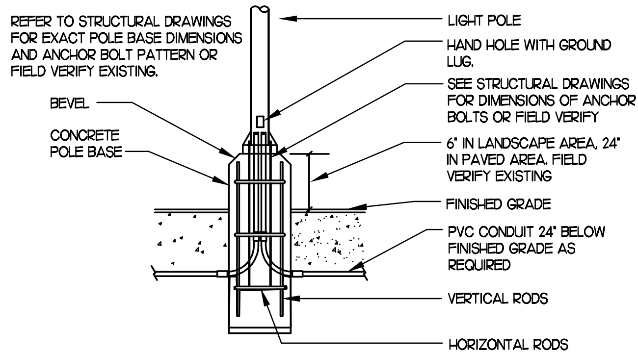
TYPICAL POLE BASE DETAIL NOT TO SCALE - FIELD VERIFY EXISTING POLE BASE BEFORE CONSTRUCTION
