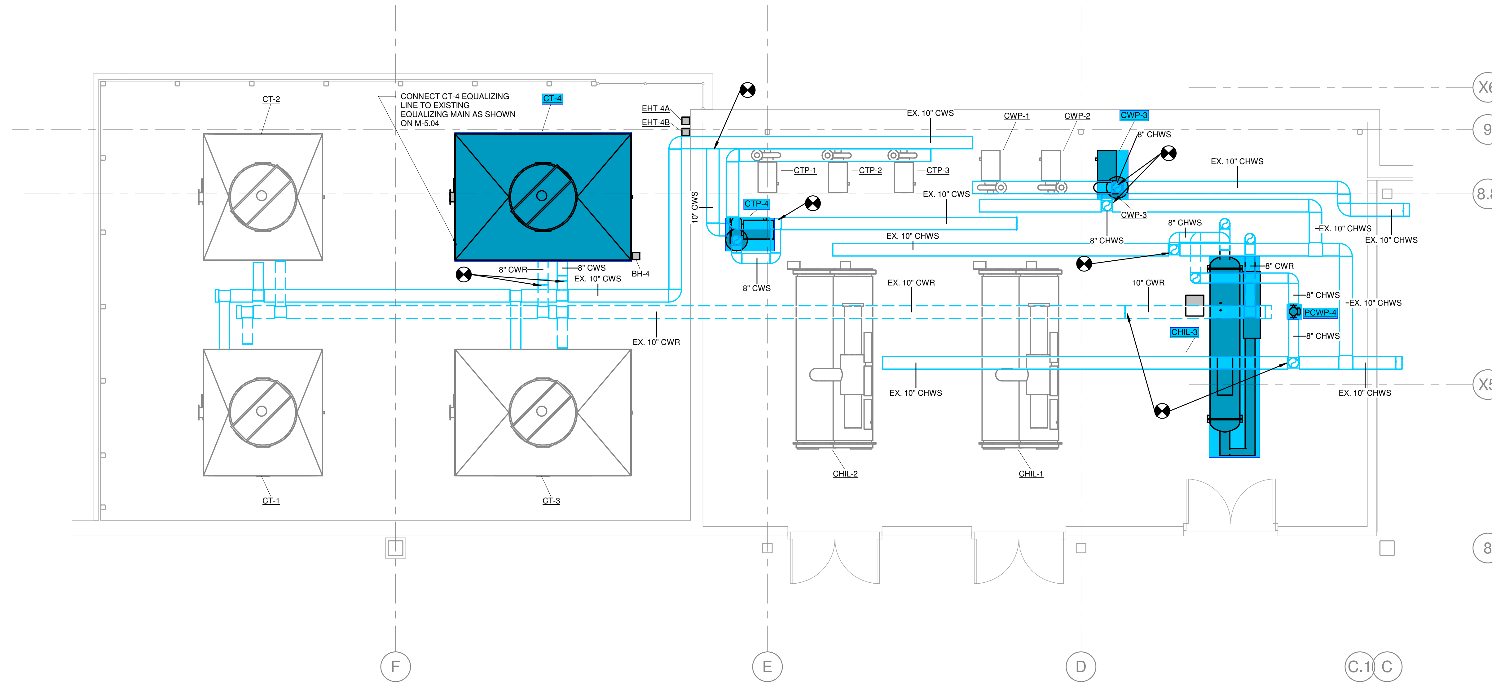
2 M-2.33 1/4" = 1'-0" MECHANICAL PIPING PLAN - ENLARGED MECHANICAL COOLING PLANT
