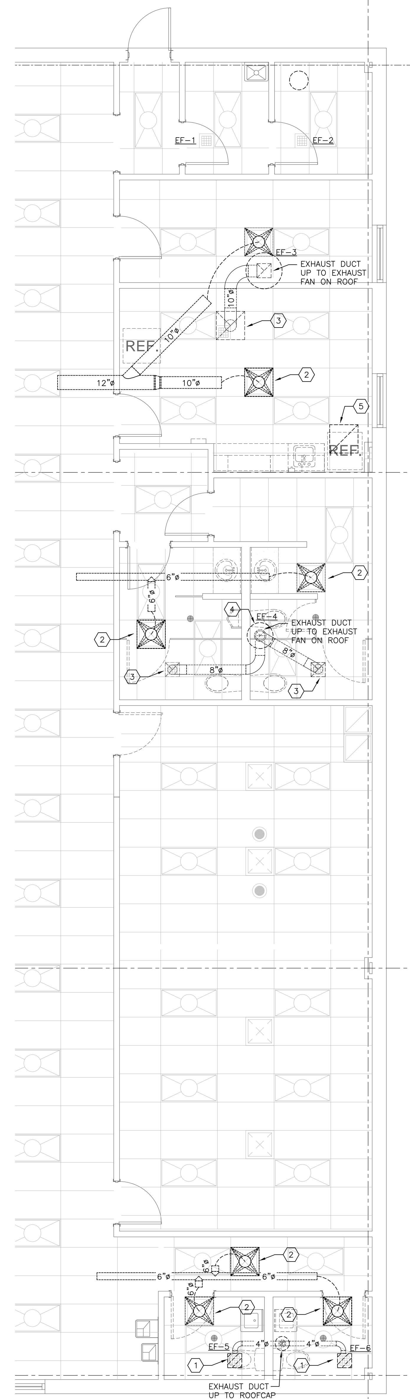
2 ENLARGED HVAC DEMOLITION PLAN M011 SCALE: 1/4" = 1'-0"
