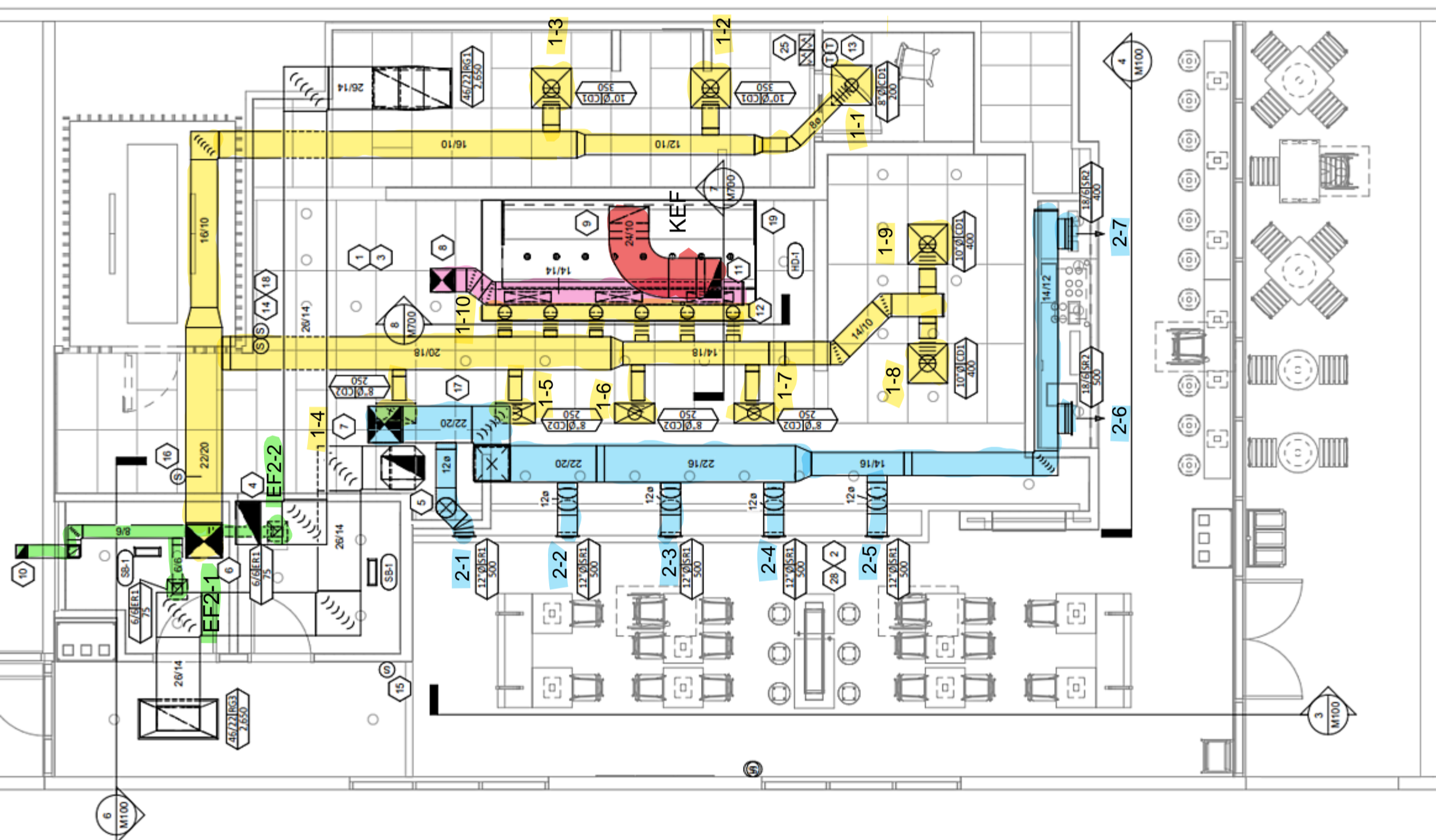
1 M100 HVAC FLOOR PLAN 1/4" = 1'-0"
