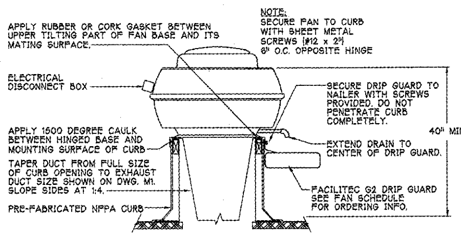
3 KITCHEN HOOD EXHAUST FAN M3 SCALE: NONE
