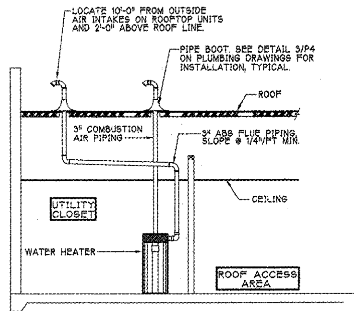
1 WATER HEATER VENT/C.A. ROUTING M3 SCALE: NONE
