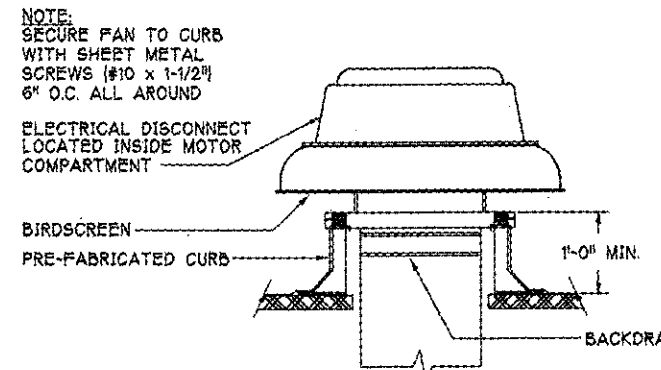
4 RESTROOM EXHAUST FAN M3 SCALE: NONE
