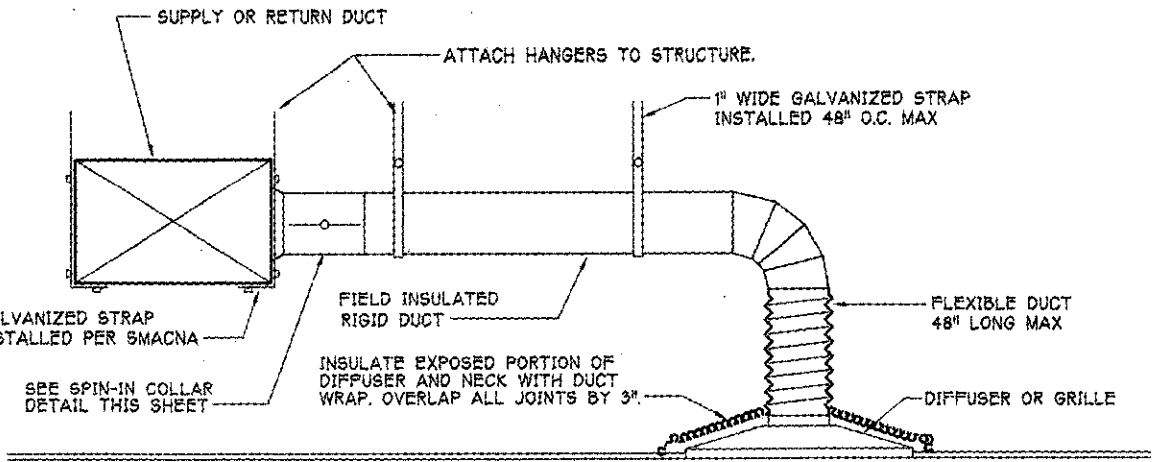
5 DIFFUSER TAKE-OFF M3 SCALE: NONE
