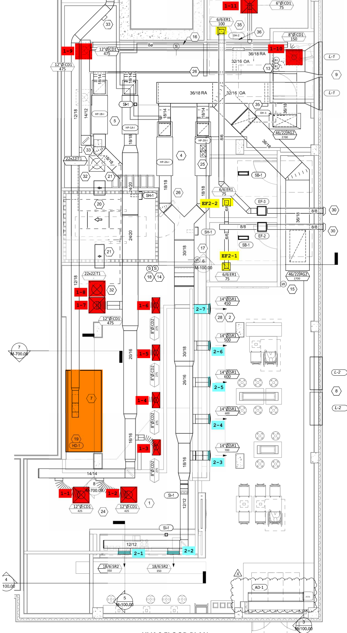
HVAC FLOOR PLAN 1/4" = 1'-0"
