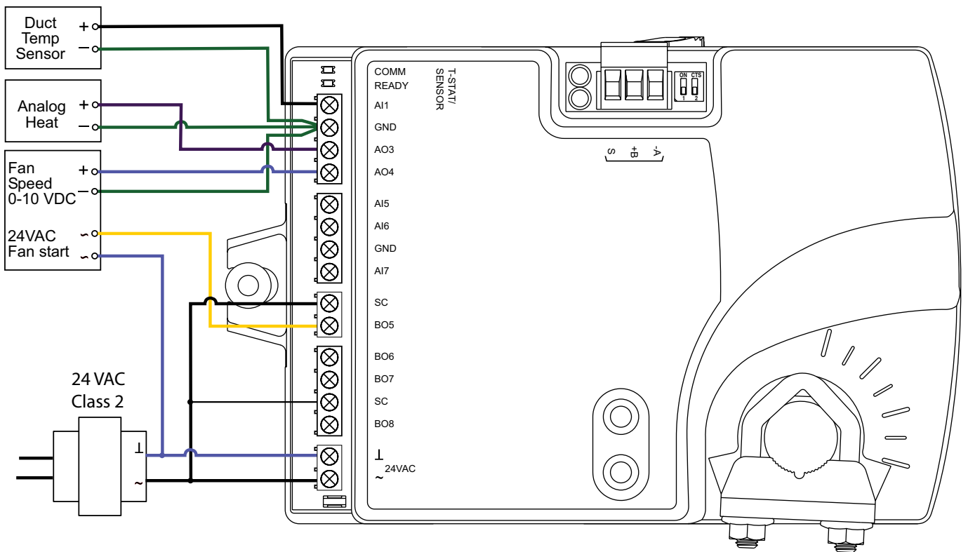
Figure 7-3 Modulating reheat
