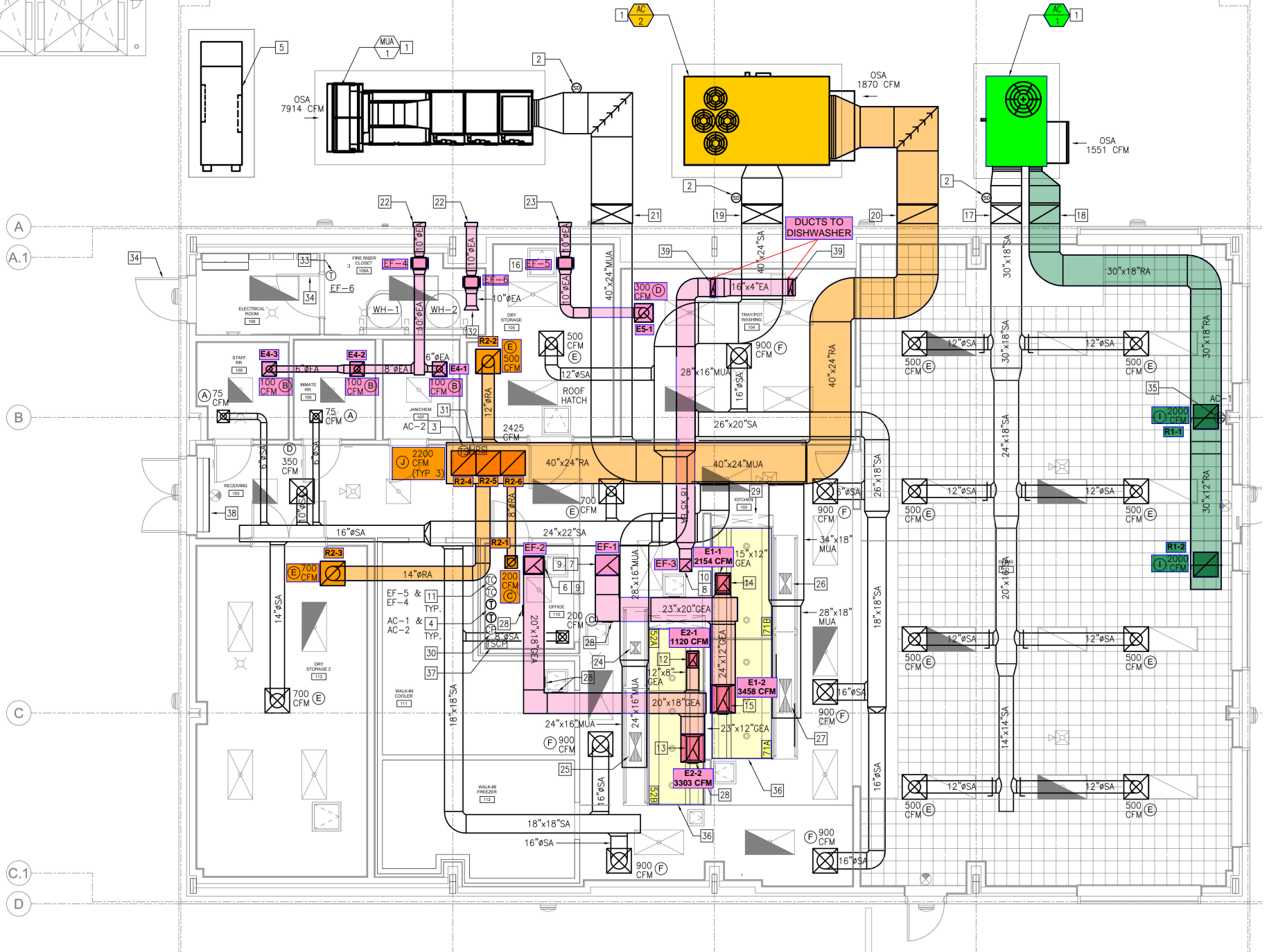
RETURN & EXHAUST
