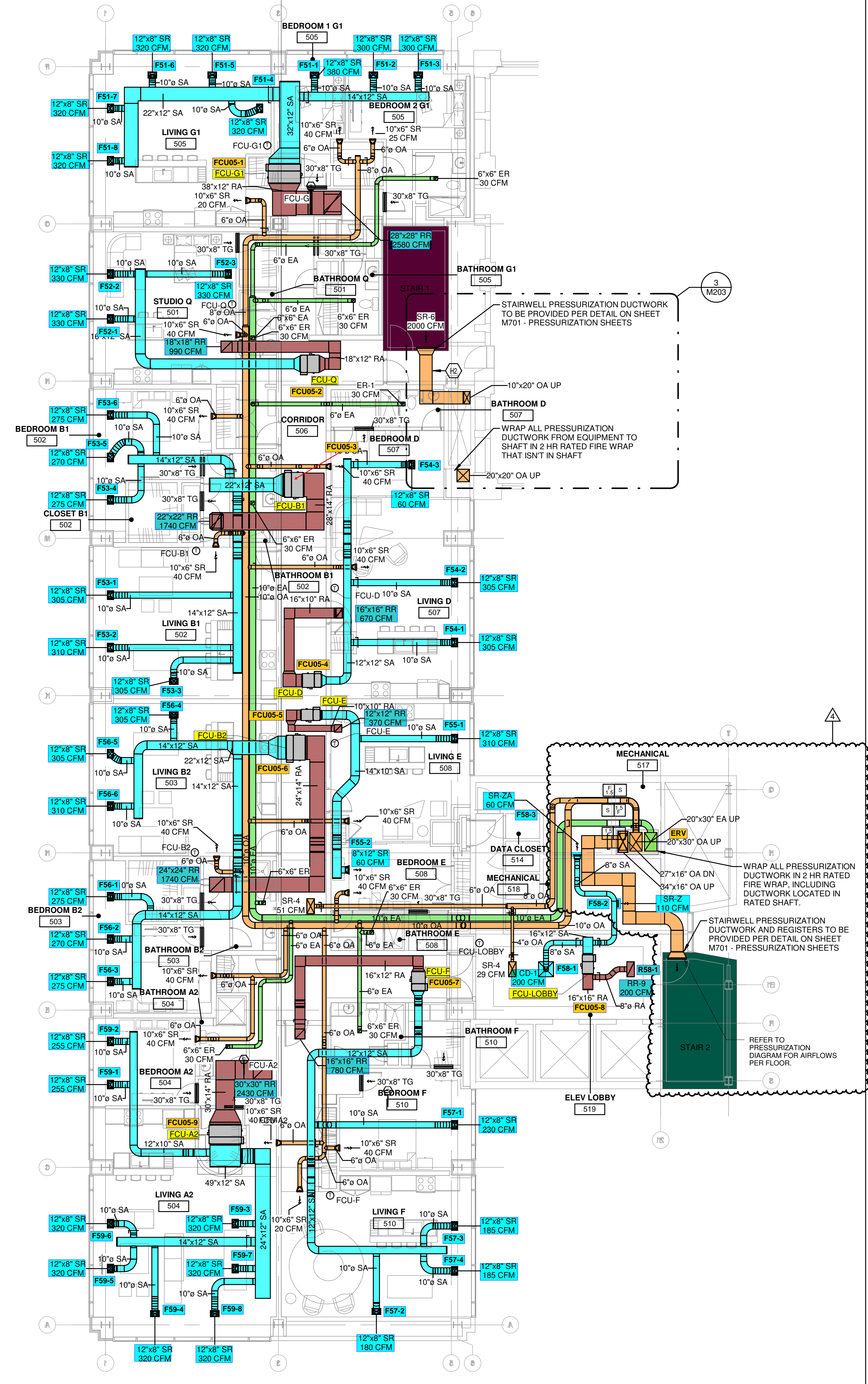
1 MECHANICAL DUCTWORK PLAN - LEVEL 5 - OVERALL 1/8" = 1'-0"
