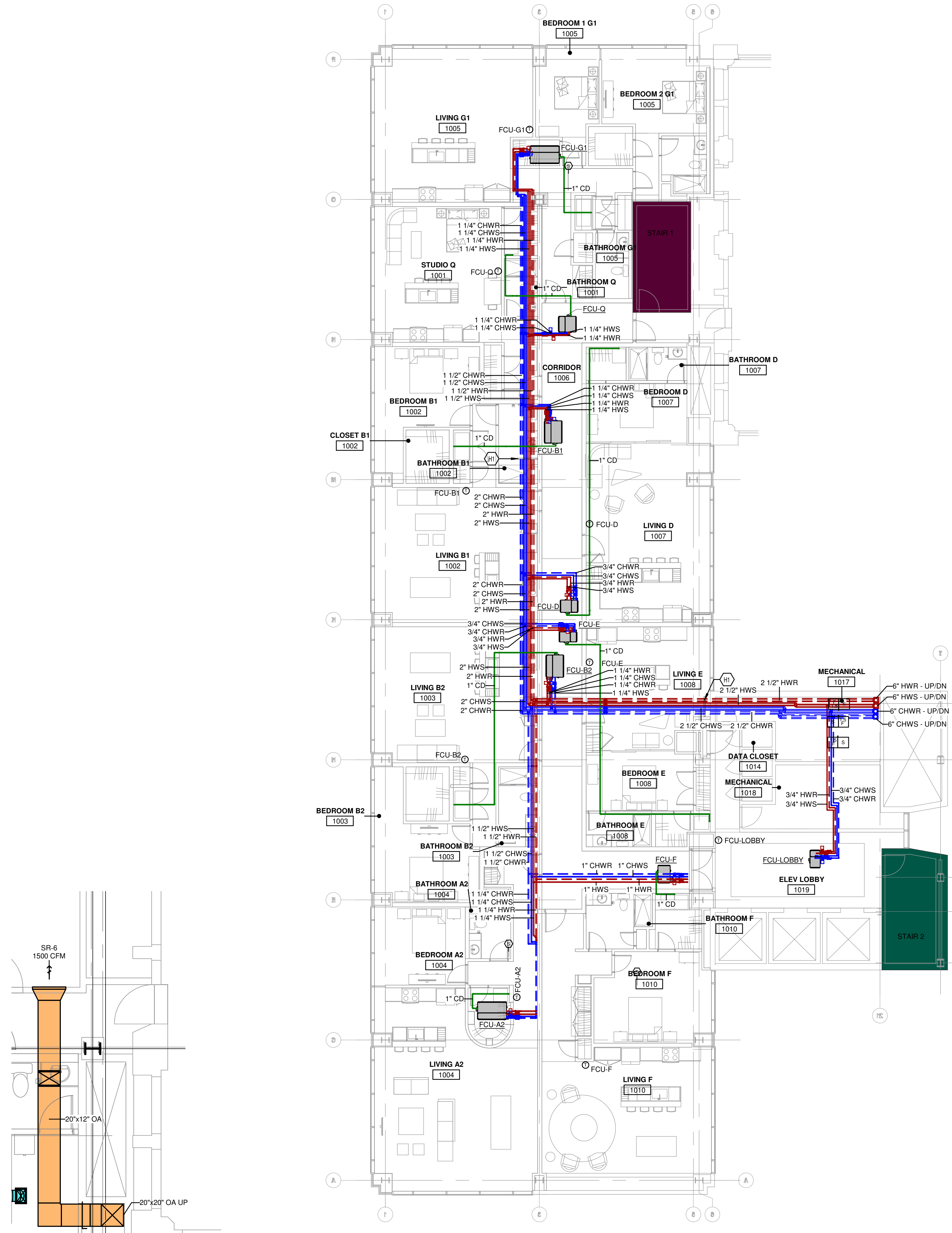
3 MECHANICAL PLAN - LEVELS 6, 4, & 3 1/4" = 1'-0"
