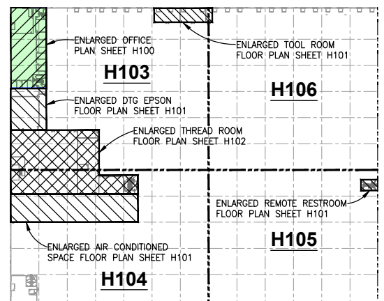
H100 - OFFICE FLOOR PLAN (PHASE 1)
