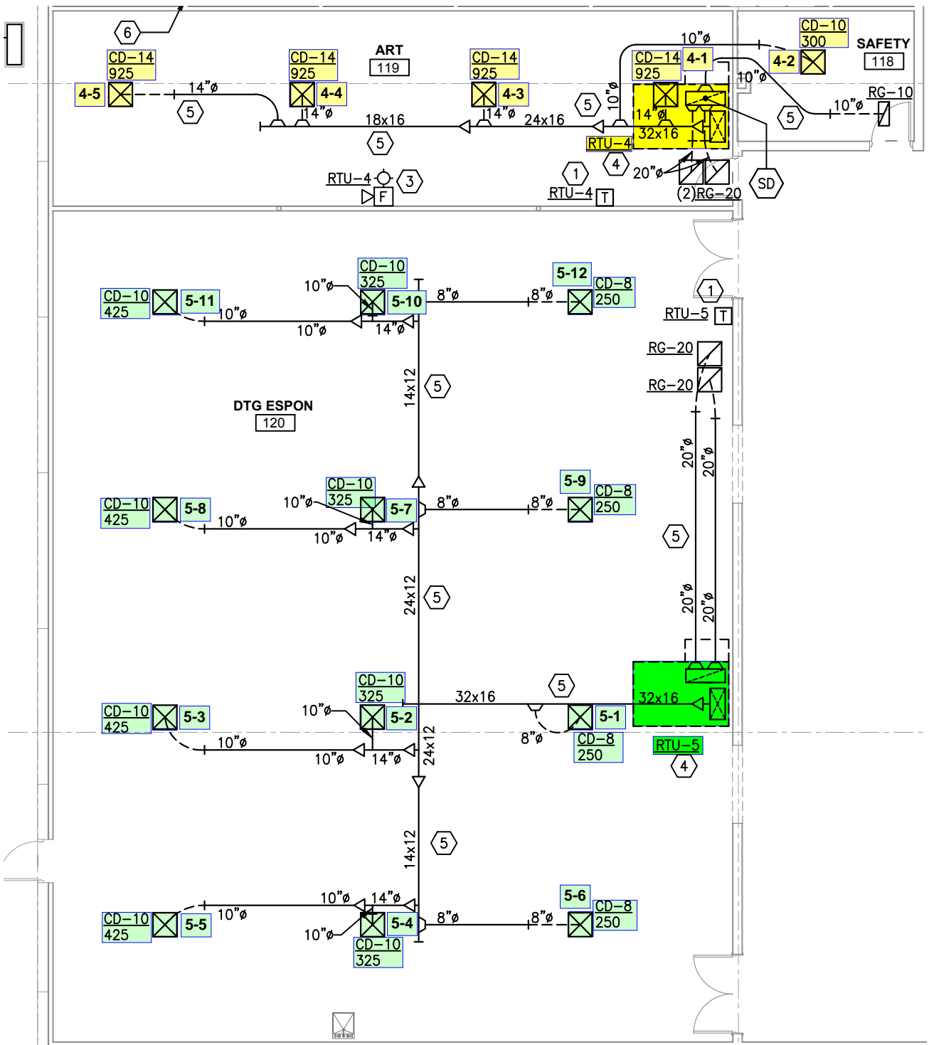
ENLARGED DTG EPSON FLOOR PLAN - HVAC
