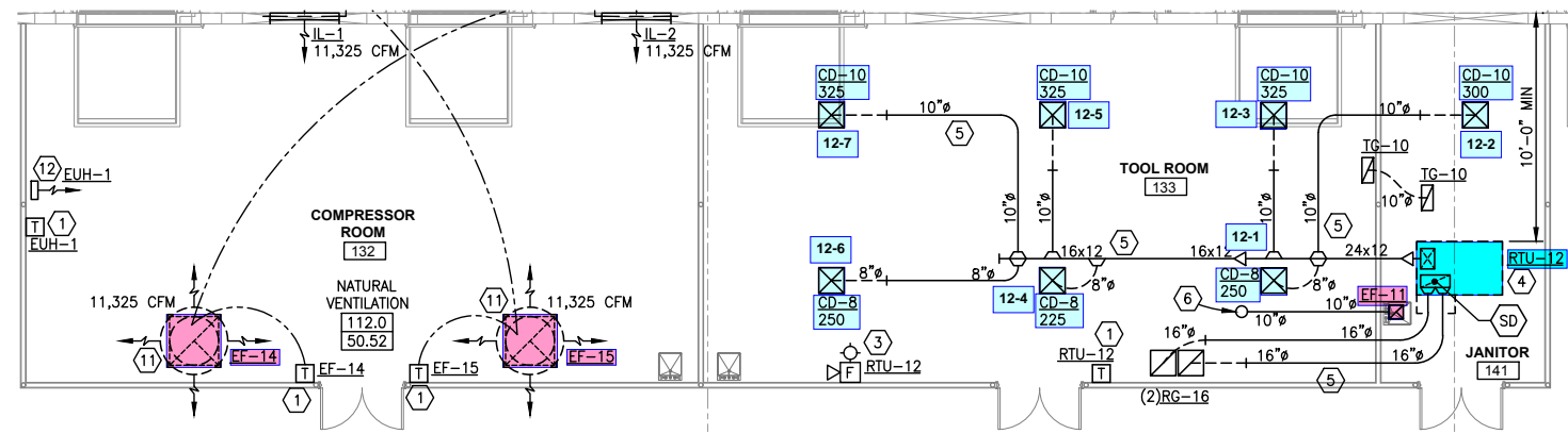
ENLARGED TOOL ROOM FLOOR PLAN - HVAC
