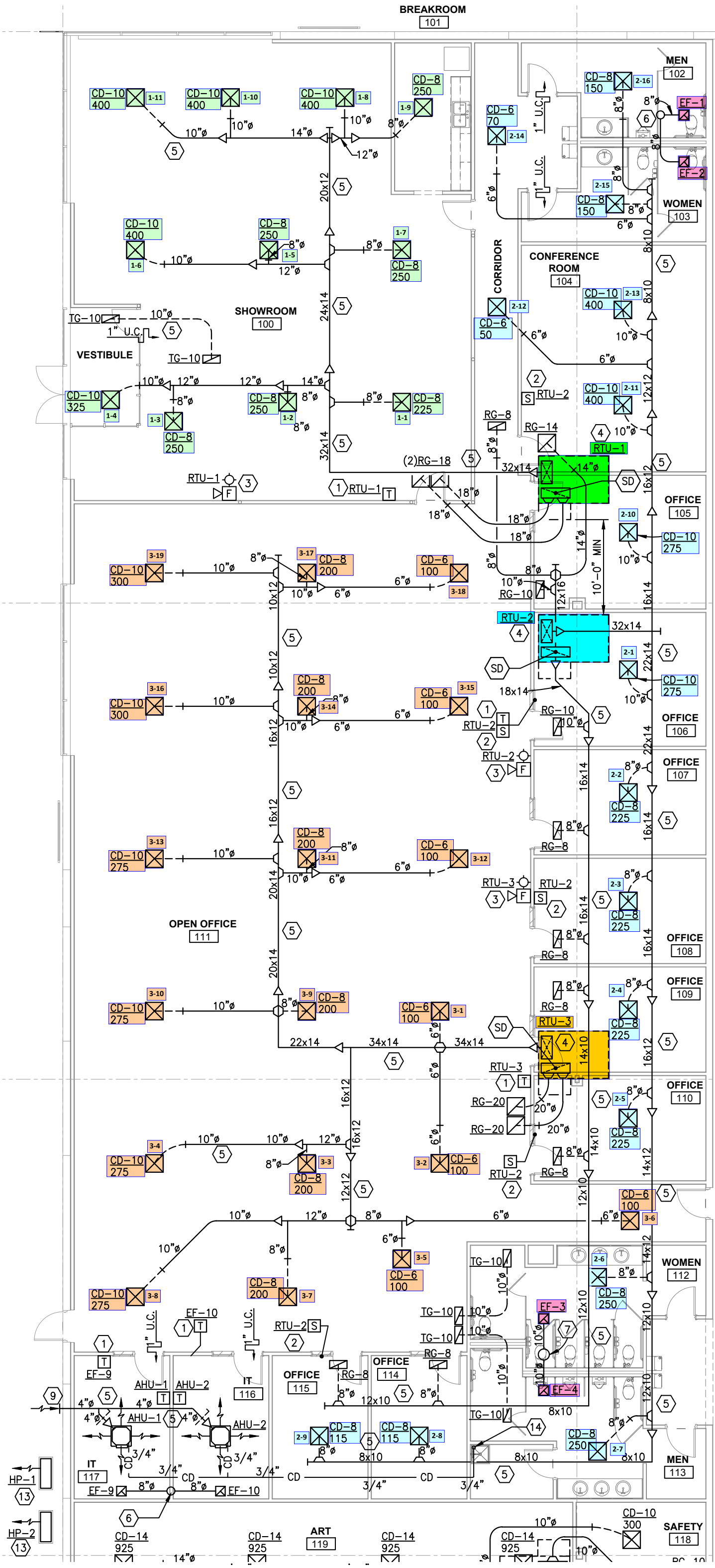
H100 - OFFICE FLOOR PLAN (PHASE 1)
