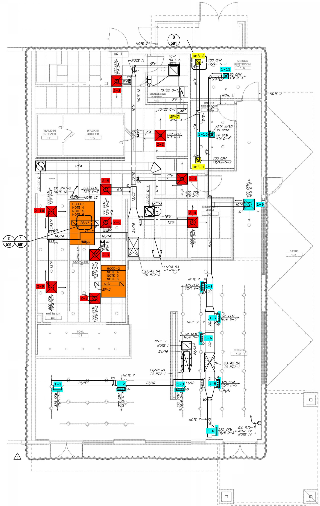
Mechanical Floor Plan
