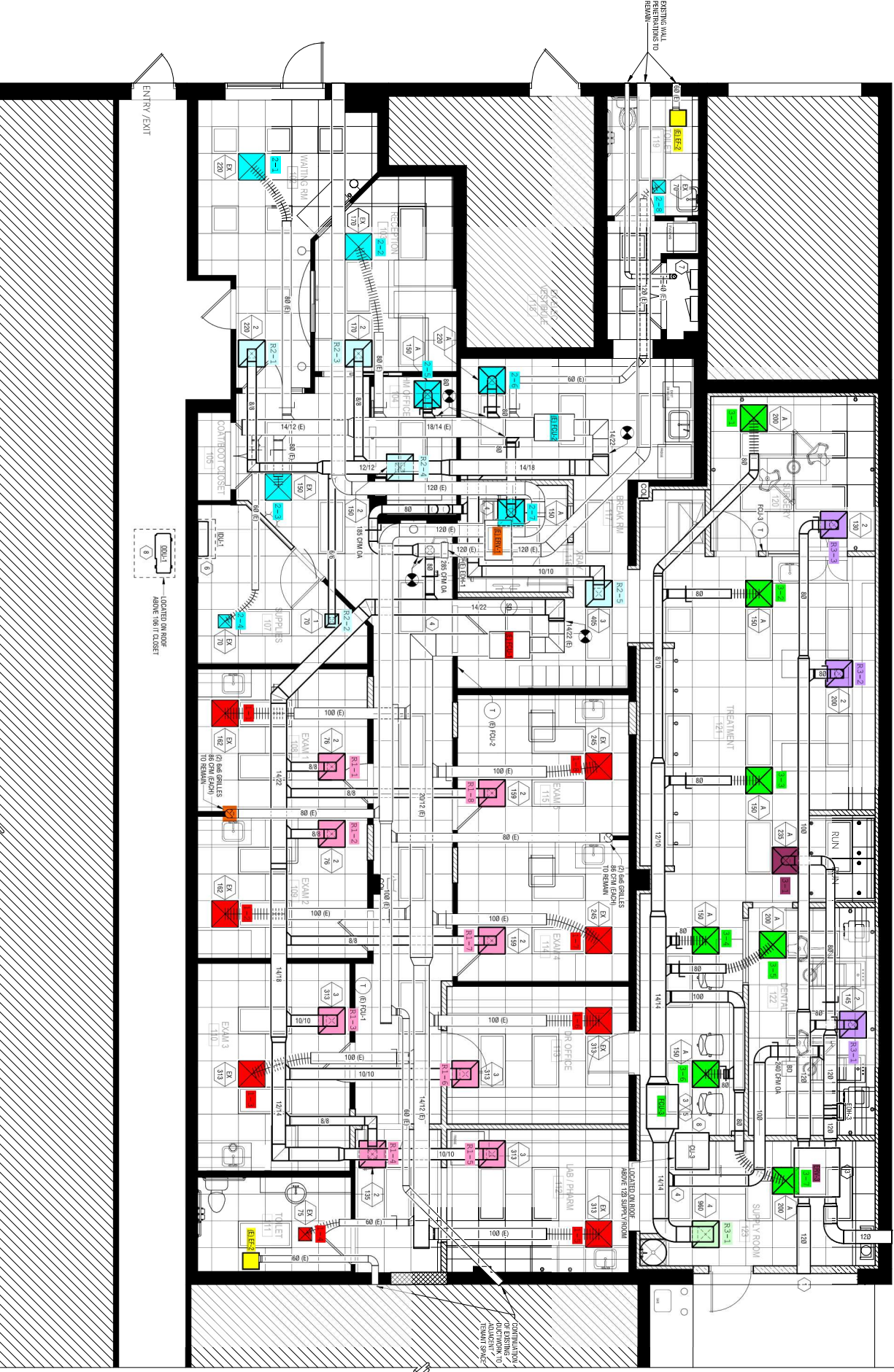
1 FIRST FLOOR DUCTWORK PLAN 1/4" = 1'-0"
