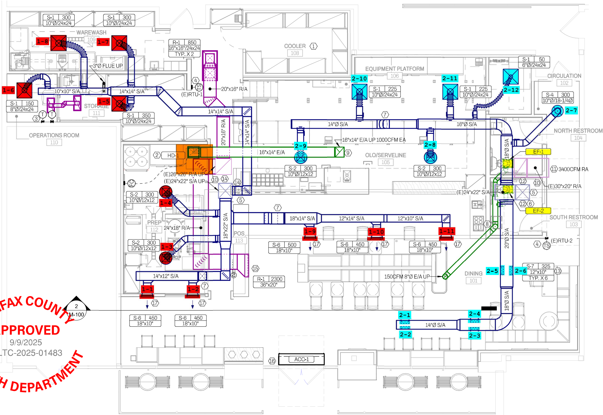
1 MECHANICAL - LEVEL 1 HVAC PLAN M-100 3/16" = 1'-0"
