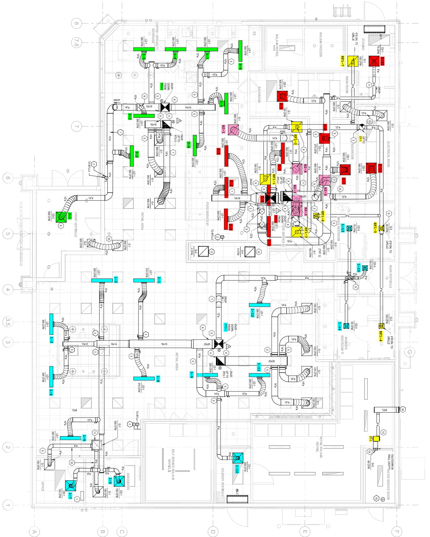
1 HVAC FLOOR PLAN 1/8" = 1'-0"
