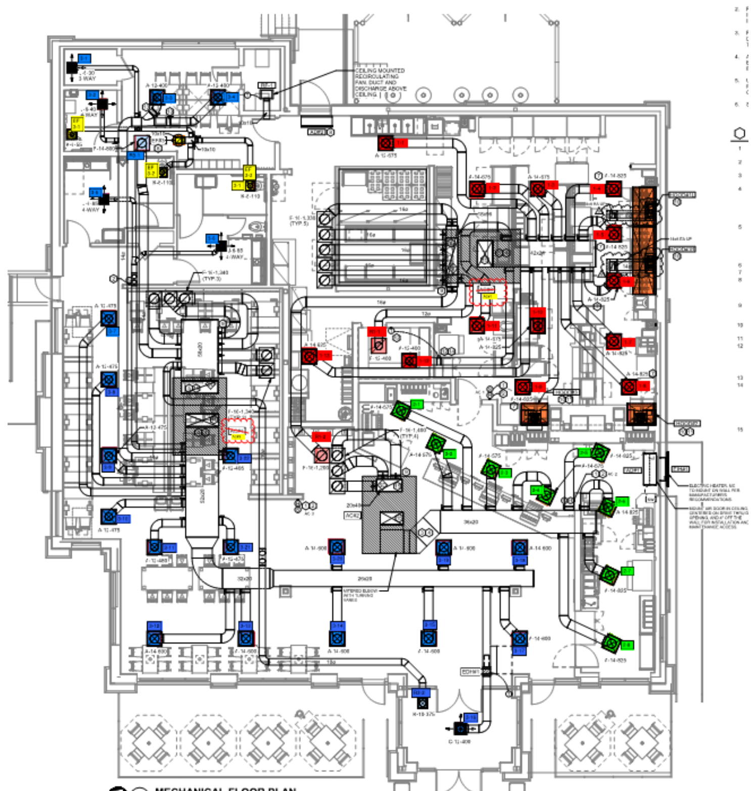
MECHANICAL FLOOR PLAN
