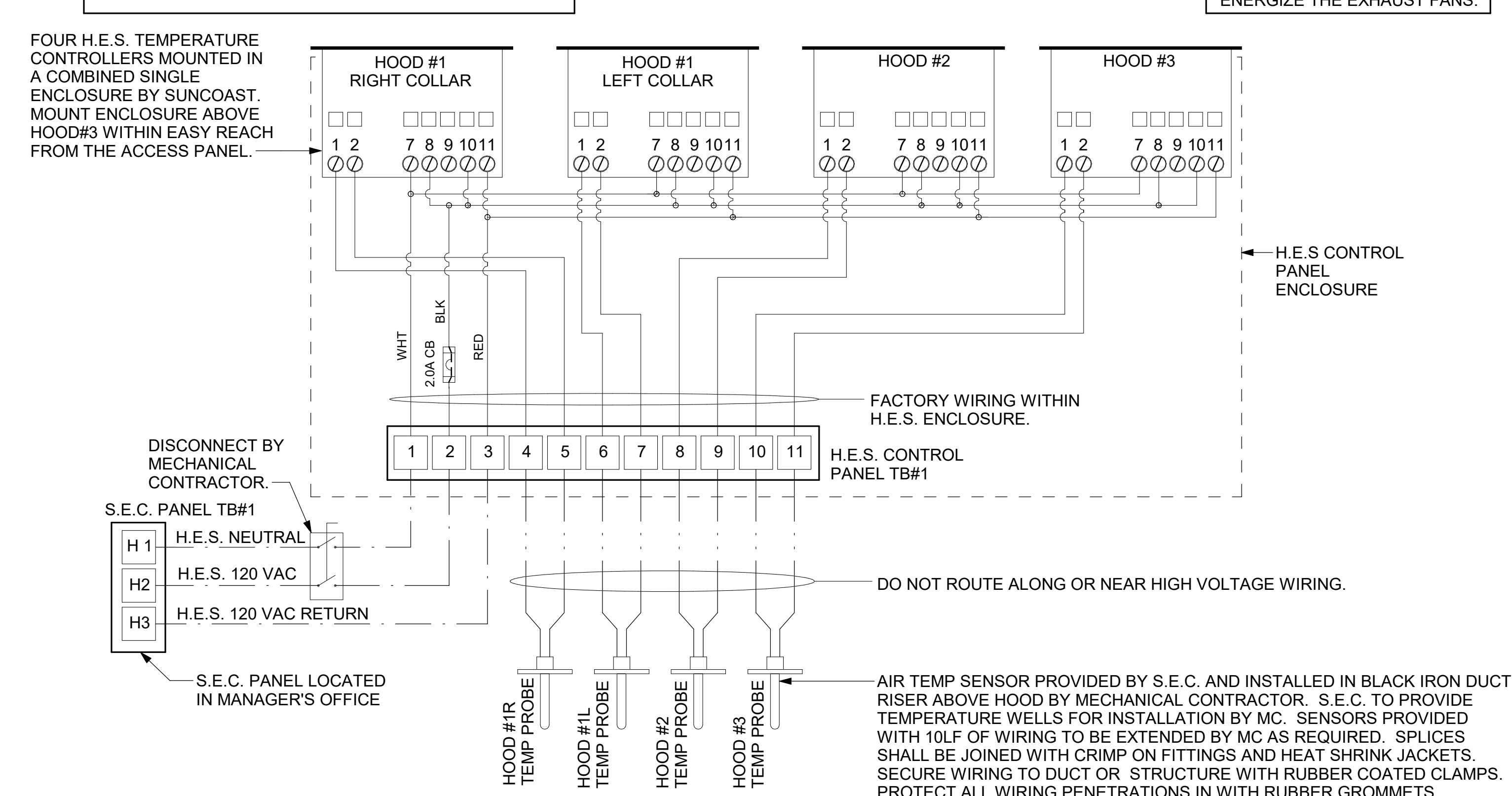
① HOOD FAN/EQUIPMENT INTERLOCK NOT TO SCALE
