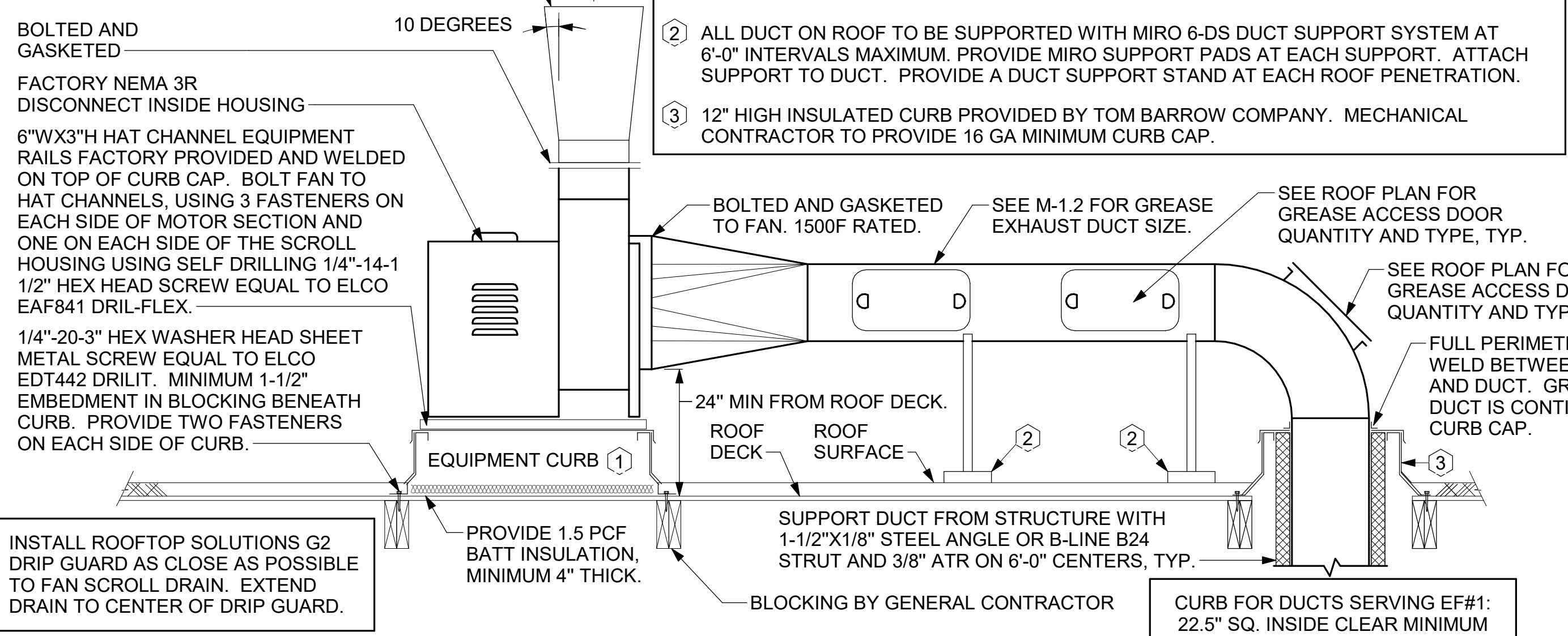
3 KITCHEN HOOD EXHAUST FANS NOT TO SCALE
