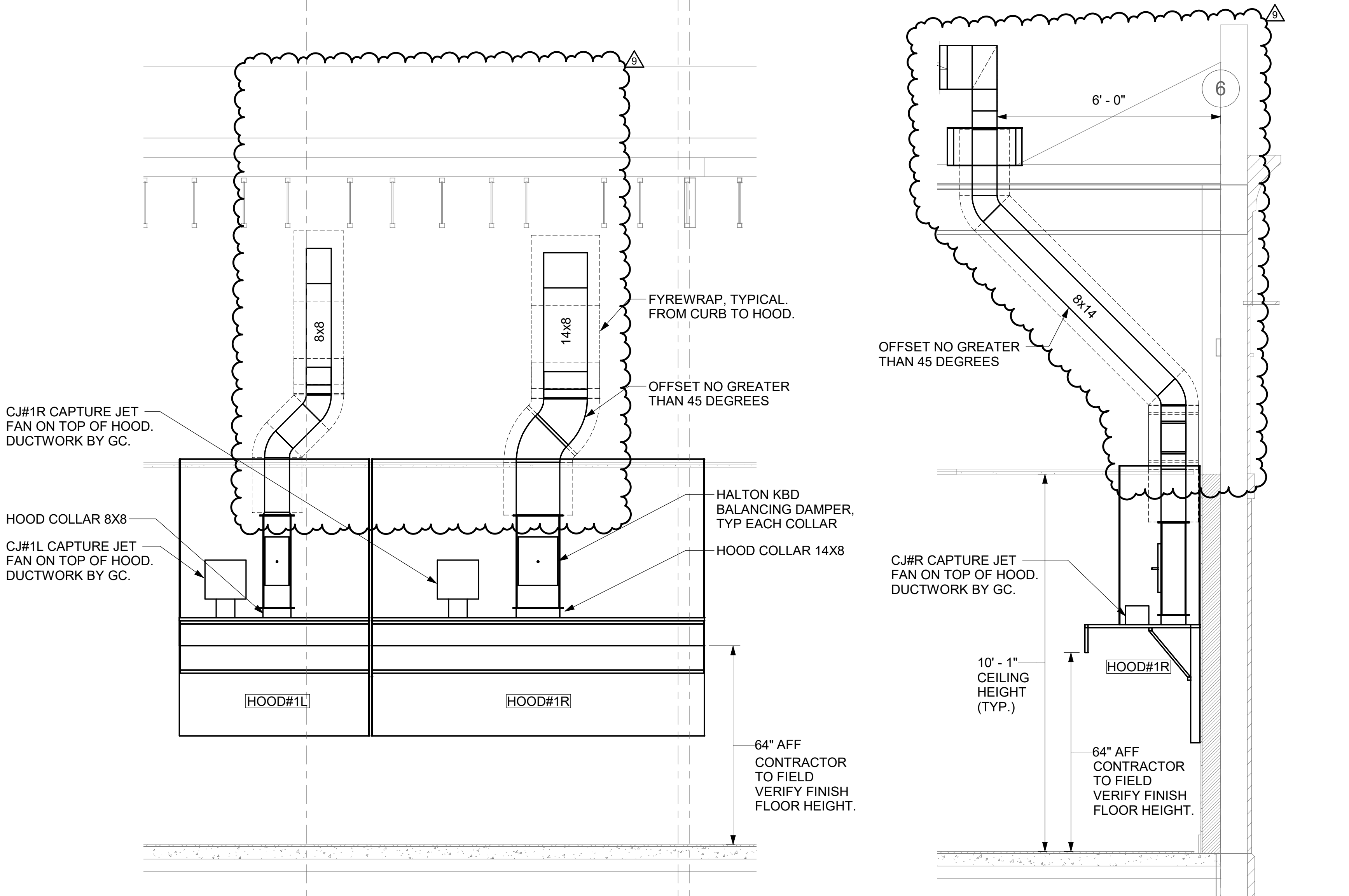
4 HOOD ELEVATION -HOOD#1 -FRONT 1/2" = 1'-0" 3 HOOD ELEVATION -HOOD#1 -SIDE 1/2" = 1'-0"
