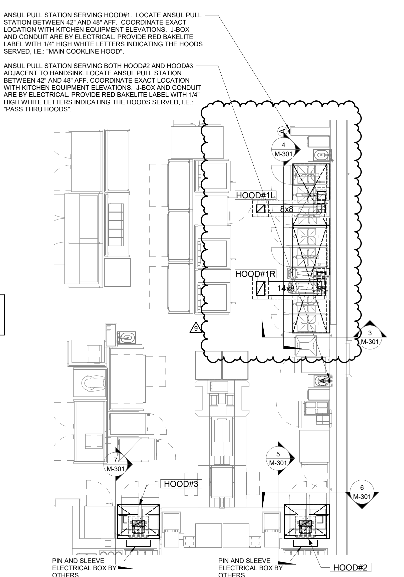
1 HOOD LAYOUT 1/4" = 1'-0"
