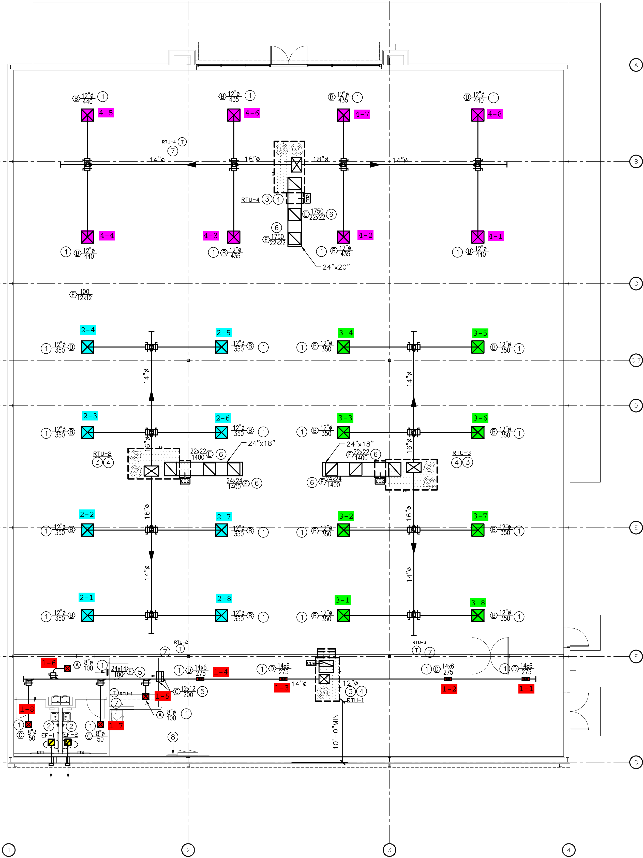
1 MECHANICAL HVAC PLAN SCALE: 1/8" = 1'-0"
