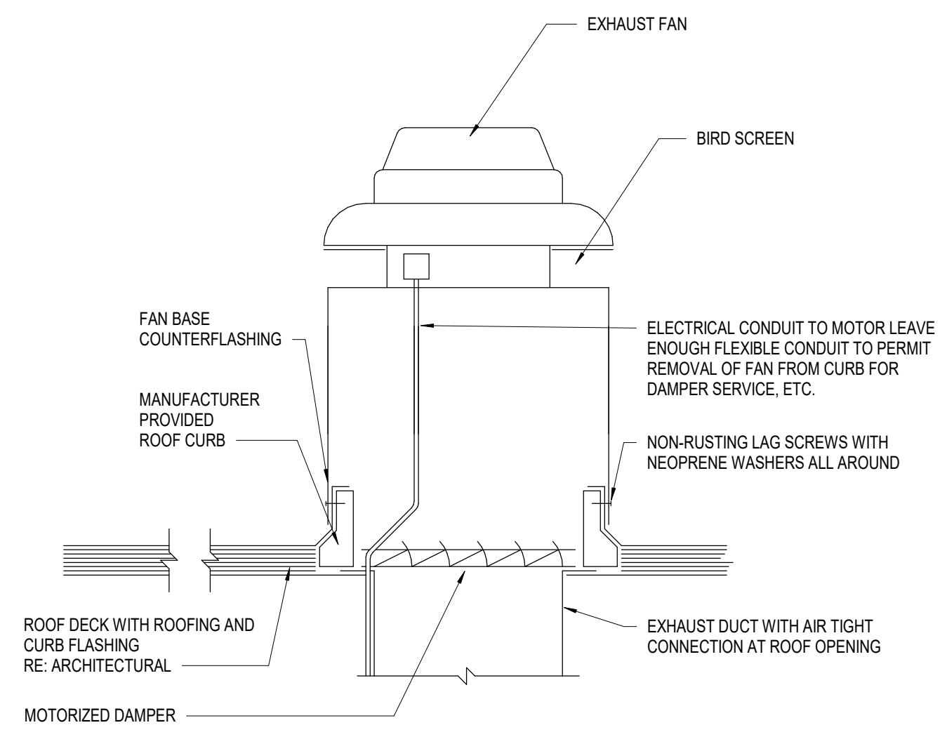
A1 ROOF MOUNTED EXHAUST FAN AND CURB DETAIL N.T.S.
