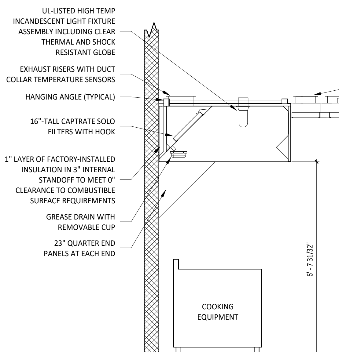
HOOD SECTION VIEW NOT TO SCALE
