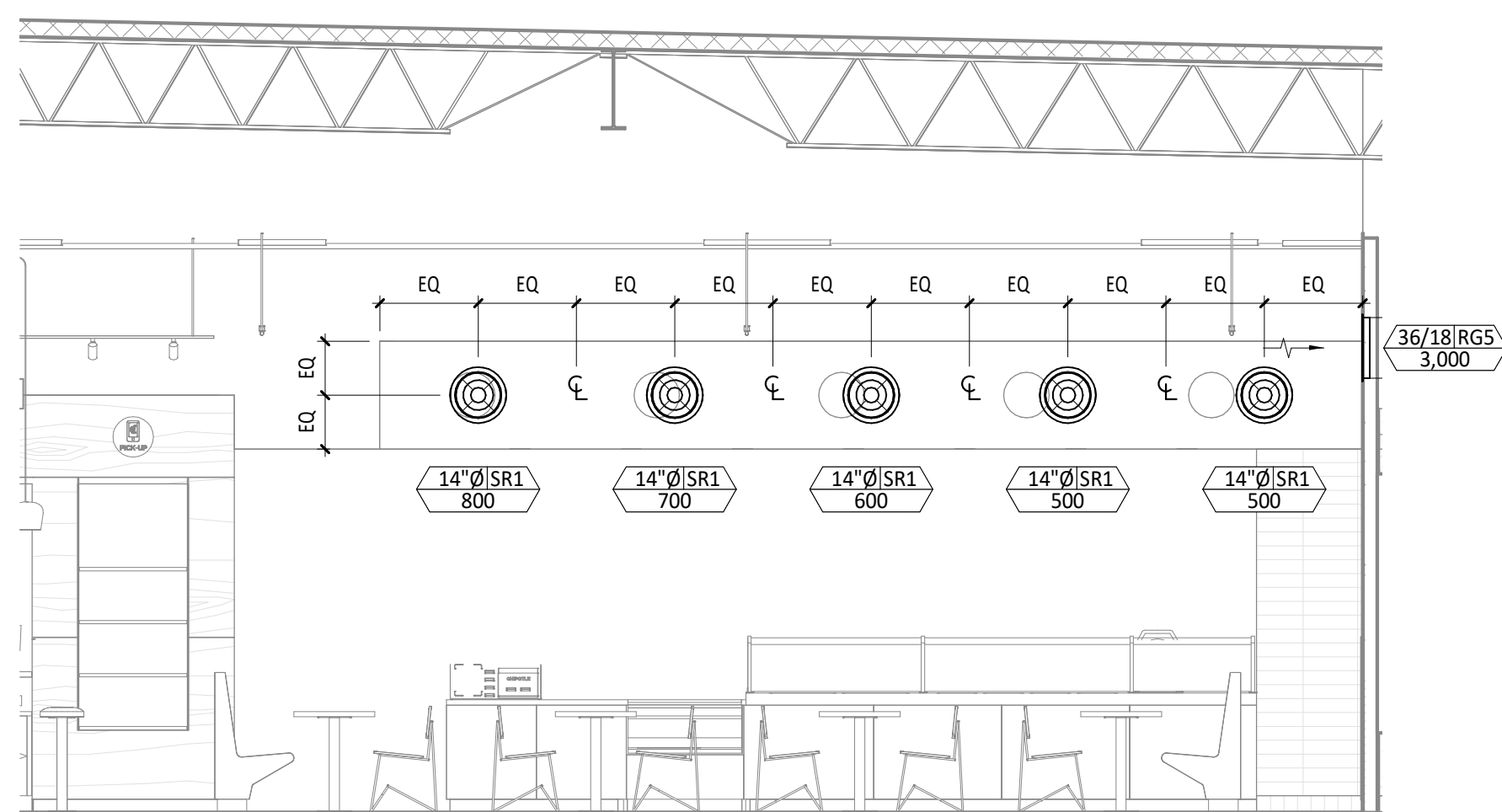
3 M100 1/4" = 1'-0" HVAC DINING ROOM SECTION
