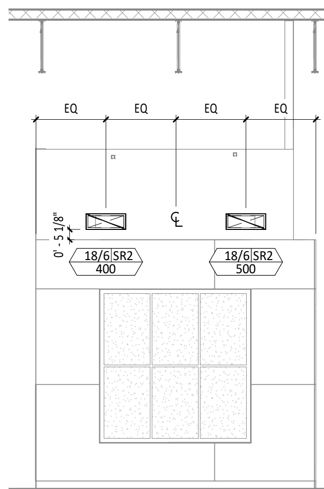
4 M100 1/4" = 1'-0" HVAC DINING ROOM SECTION
