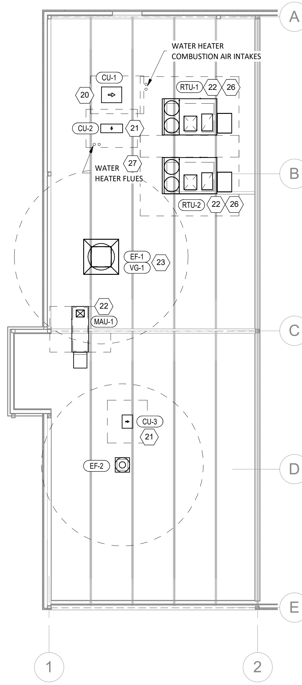
2 M100 1/8" = 1'-0" HVAC ROOF PLAN
