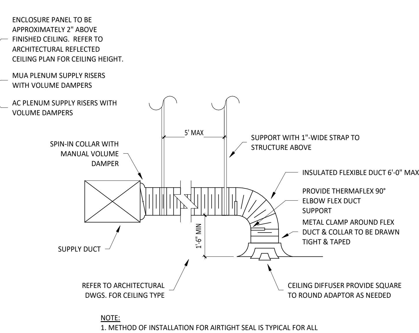
DIFFUSER CONNECTION NOT TO SCALE
