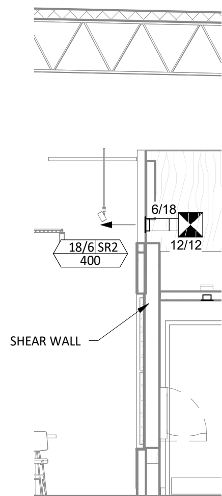
5 M100 1/4" = 1'-0" HVAC DINING ROOM SECTION
