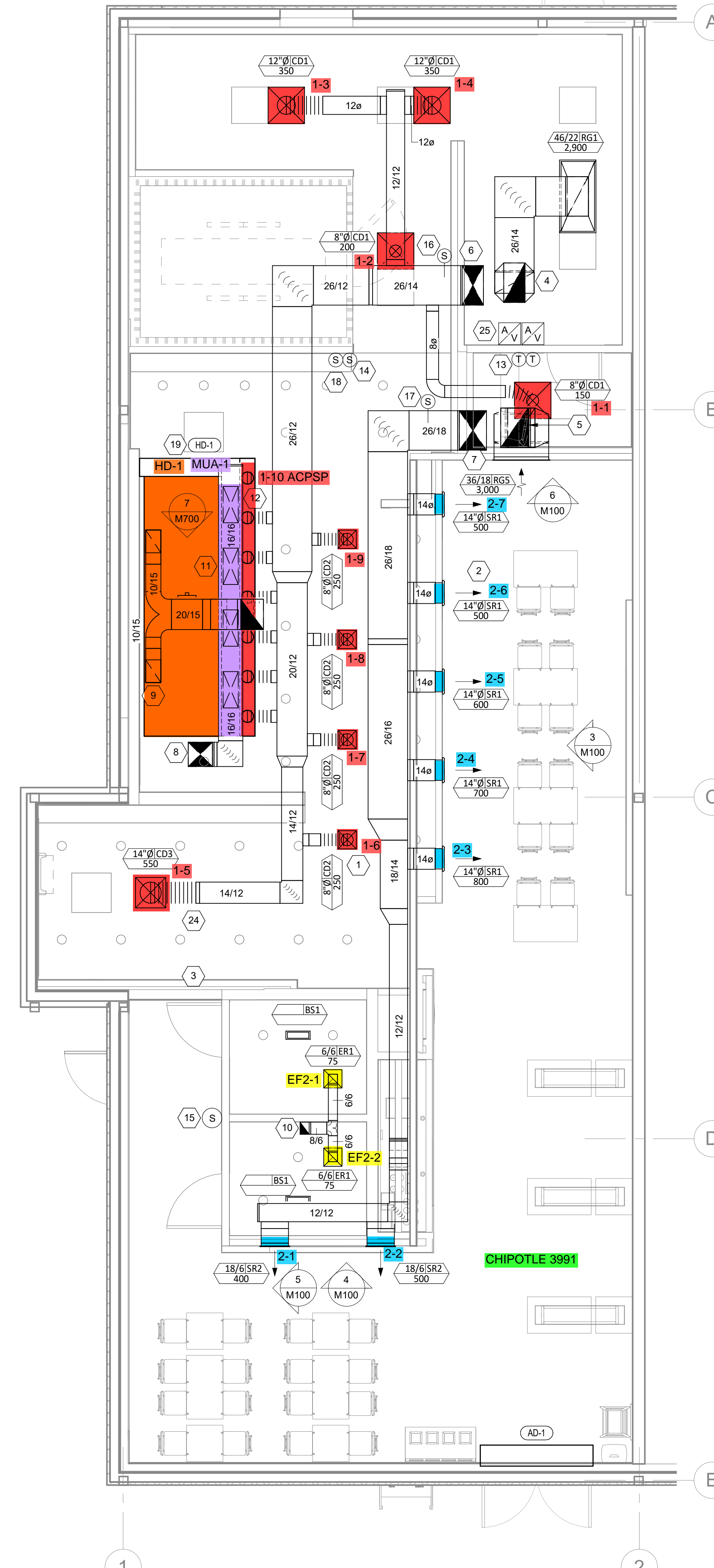
1 M100 1/4" = 1'-0" HVAC FLOOR PLAN
