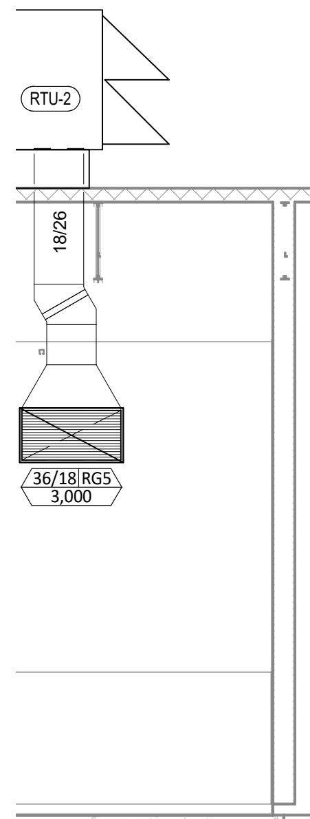
6 M100 1/4" = 1'-0" HVAC DINING ROOM RETURN SECTION
