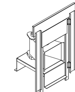
DIRECT FIRED (DF) PROFILE PLATE ASSEMBLY
