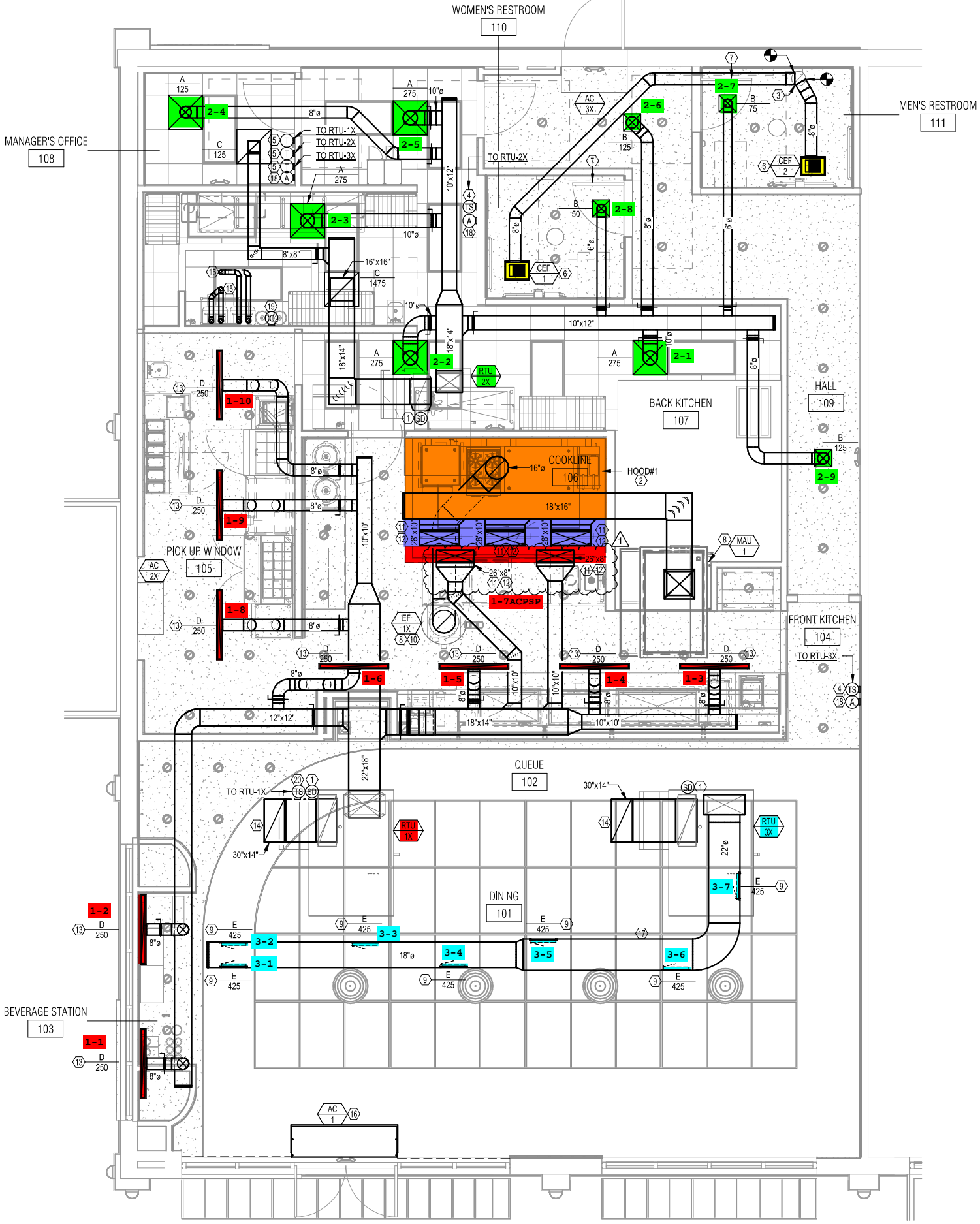
MECHANICAL PLAN SCALE: 1/4" = 1'-0"
