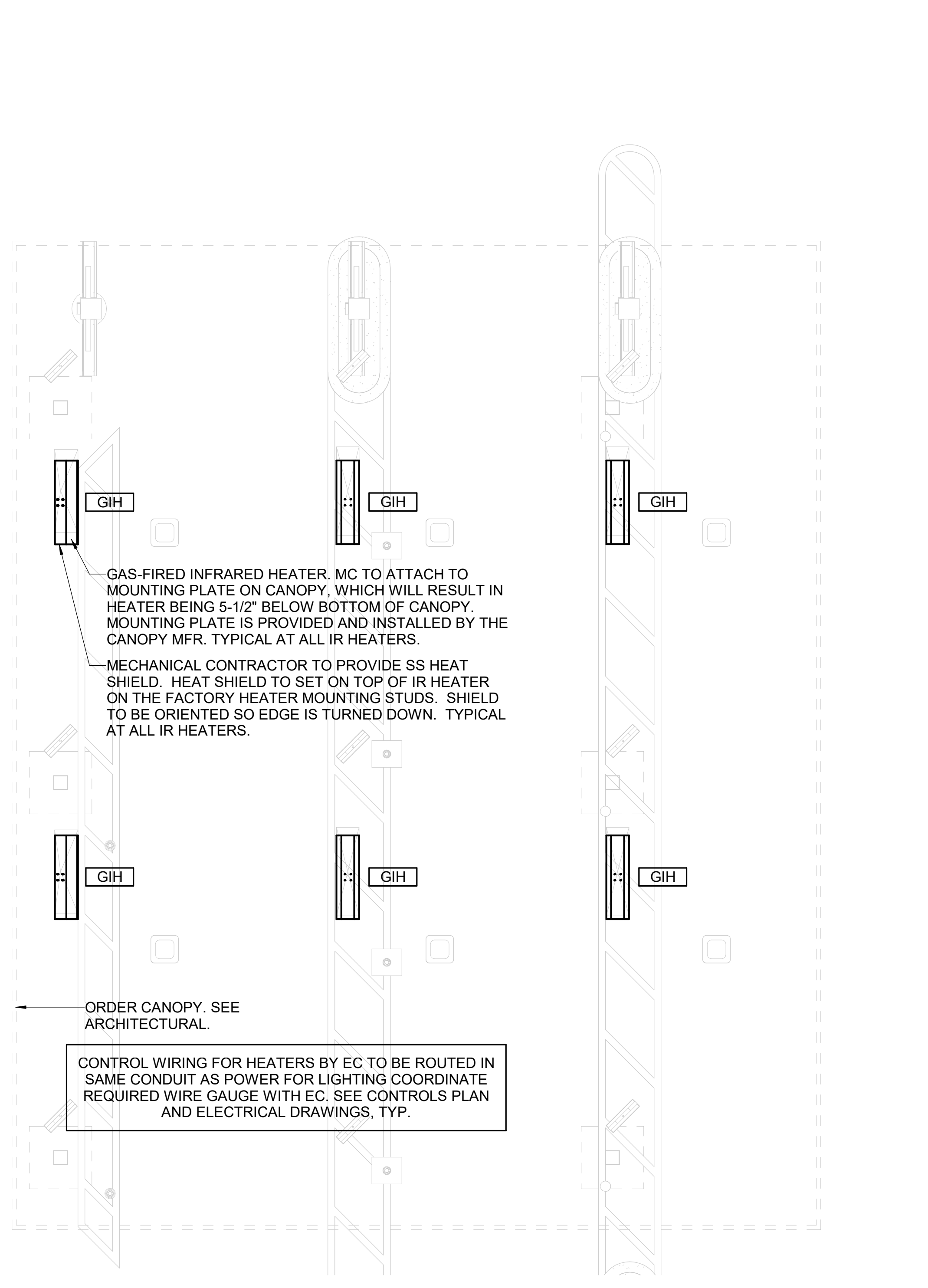
2 MECHANICAL FLOOR PLAN 1/4" = 1'-0"
