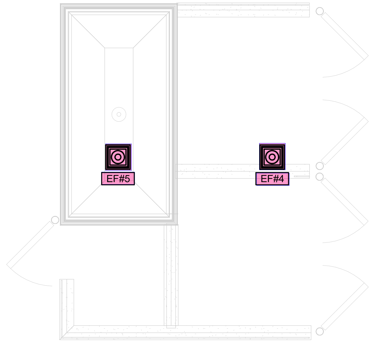
2 TRASH ENCLOSURE ROOF PLAN 1/4" = 1'-0"
