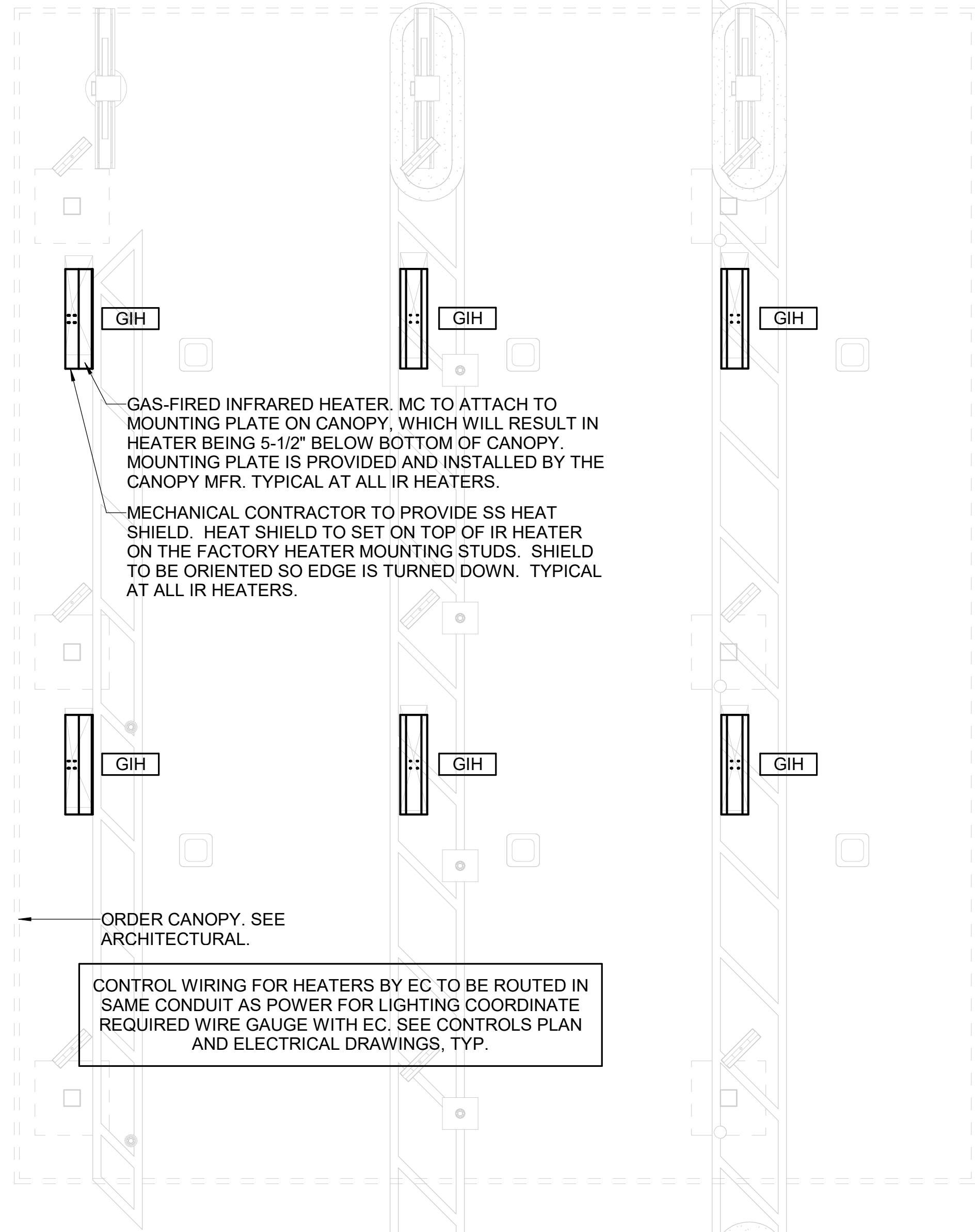
2 MECHANICAL FLOOR PLAN 1/4" = 1'-0"
