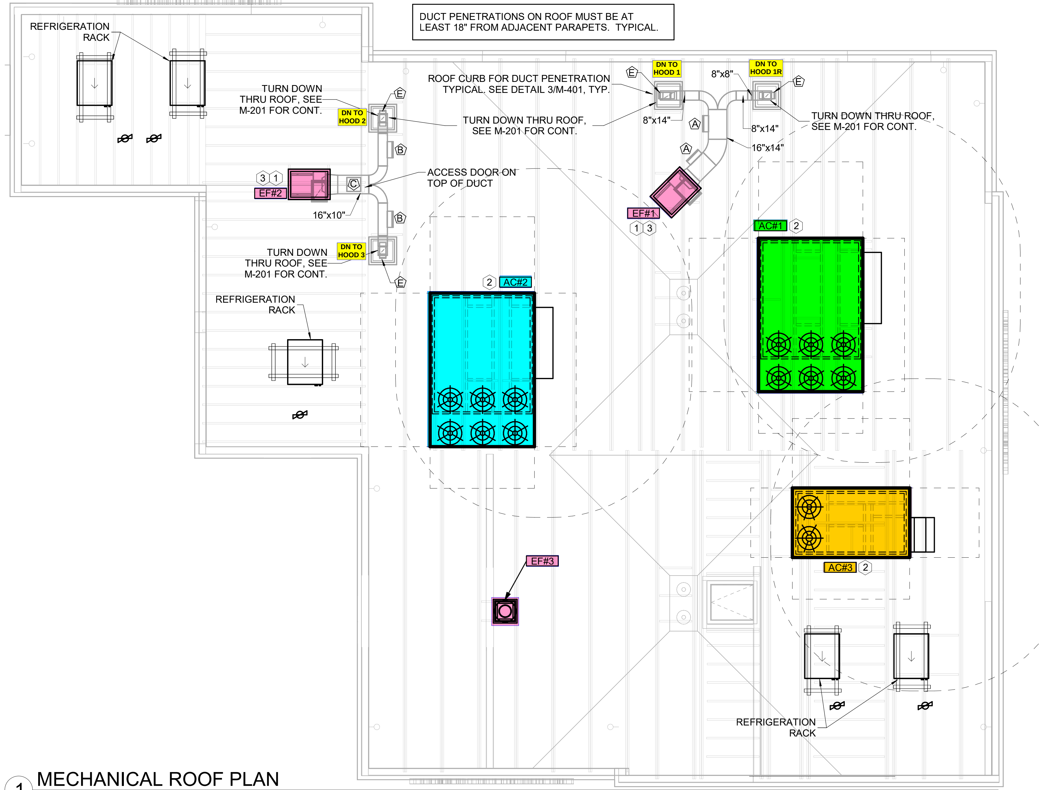
1 MECHANICAL ROOF PLAN 1/4" = 1'-0"
