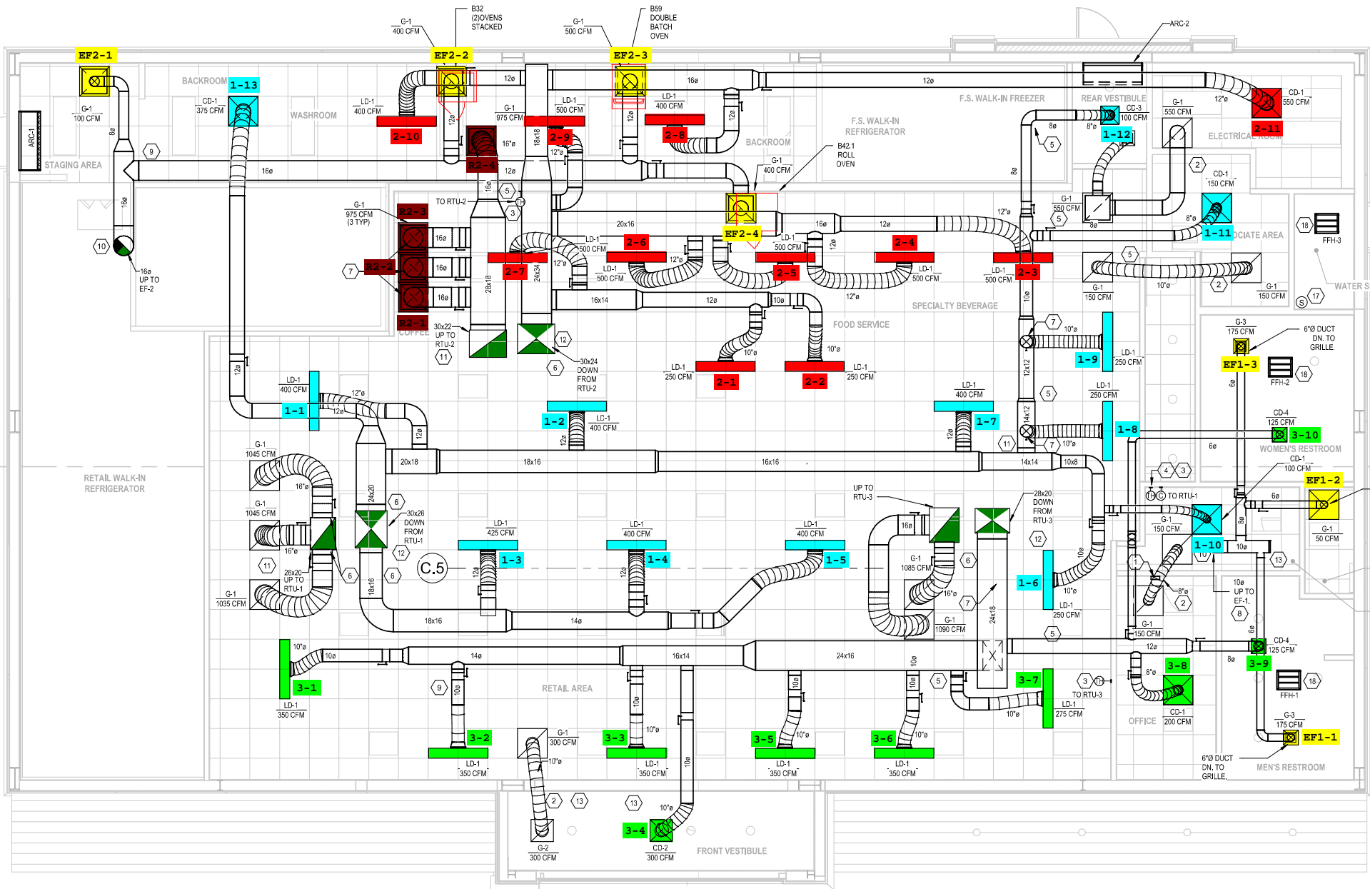
1 HVAC FLOOR PLAN M.T.O. 1/4" = 1'-0"
