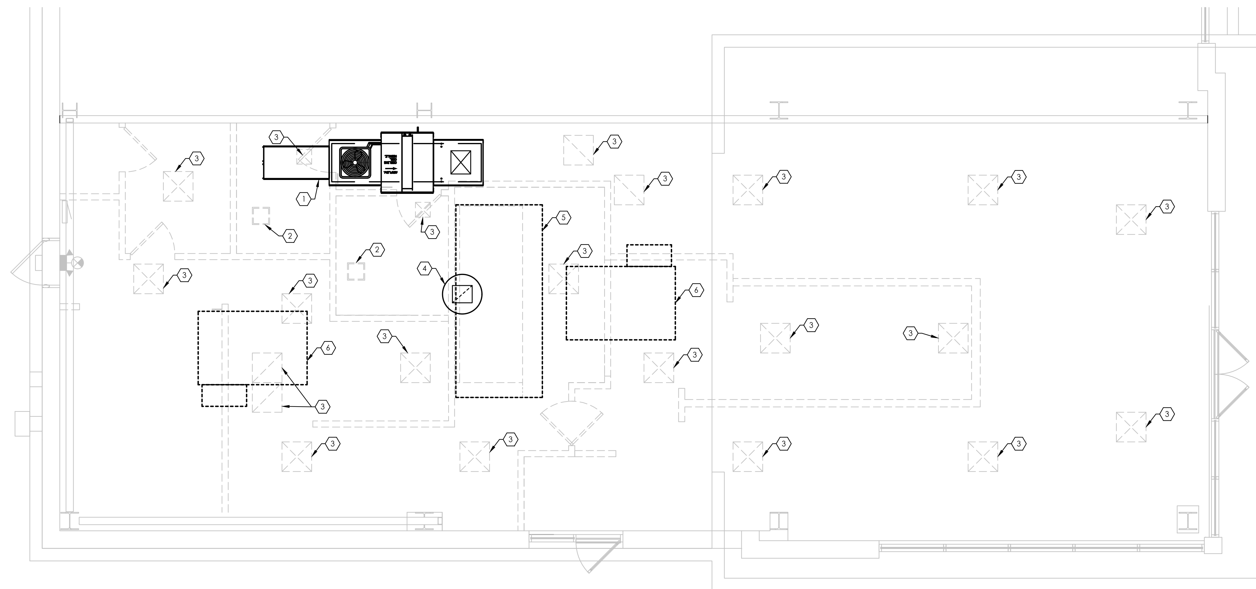
1 MECHANICAL DEMOLITION PLAN 1/4" = 1'-0"
