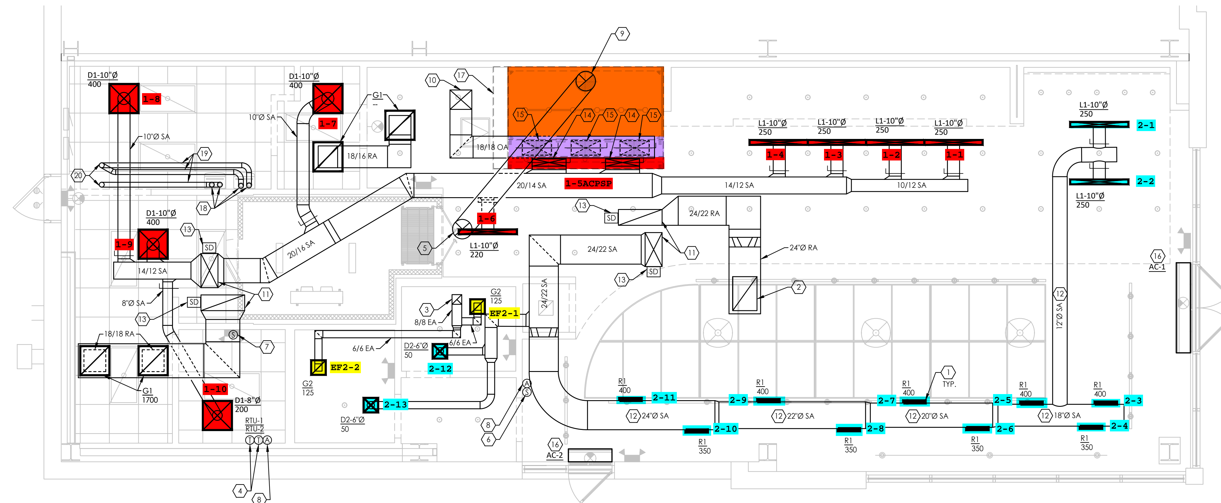
MECHANICAL PLAN 1/4" = 1'-0"
