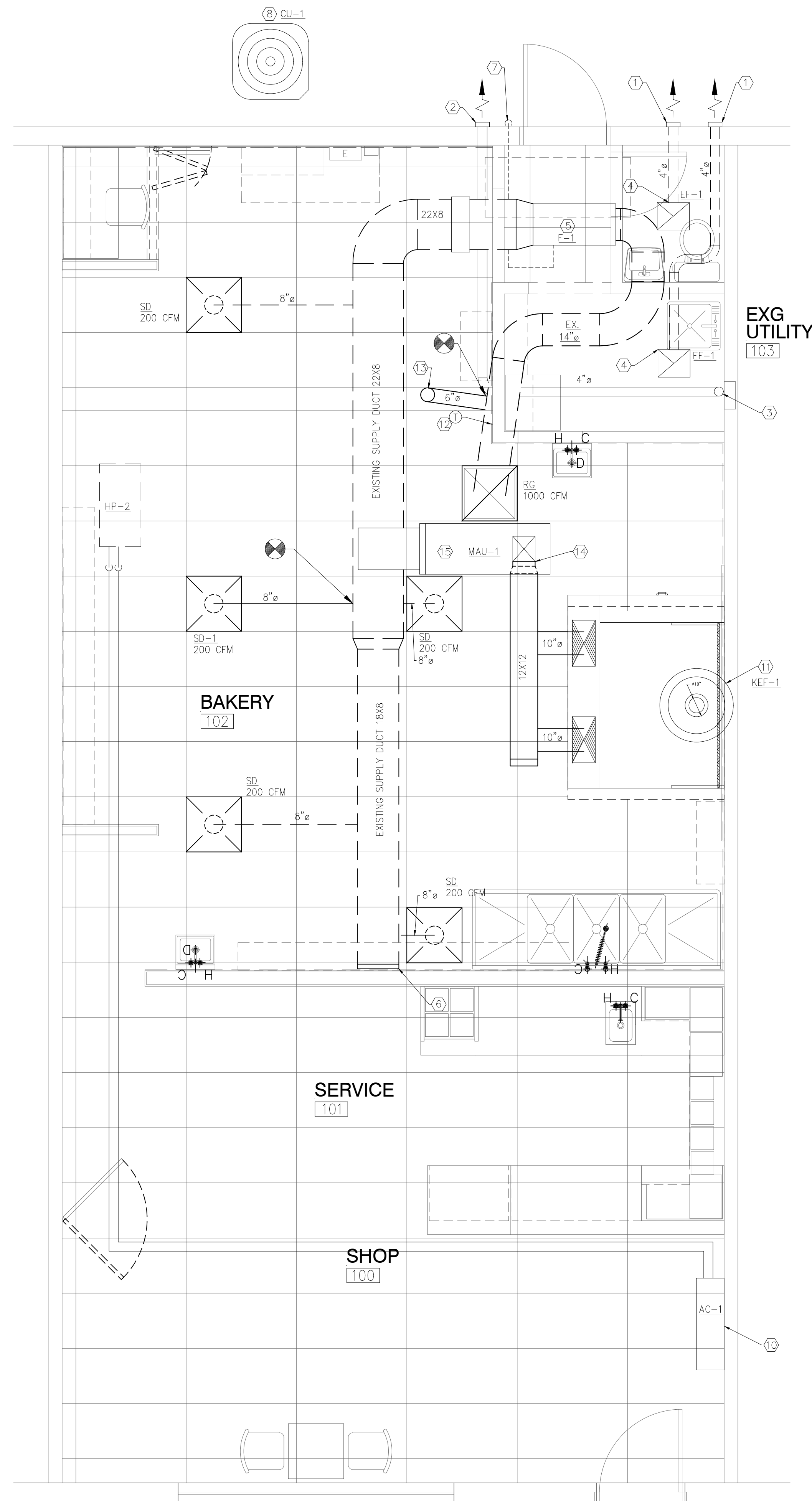
FLOOR PLAN - MECHANICAL SCALE: 3/8" = 1'-0"
