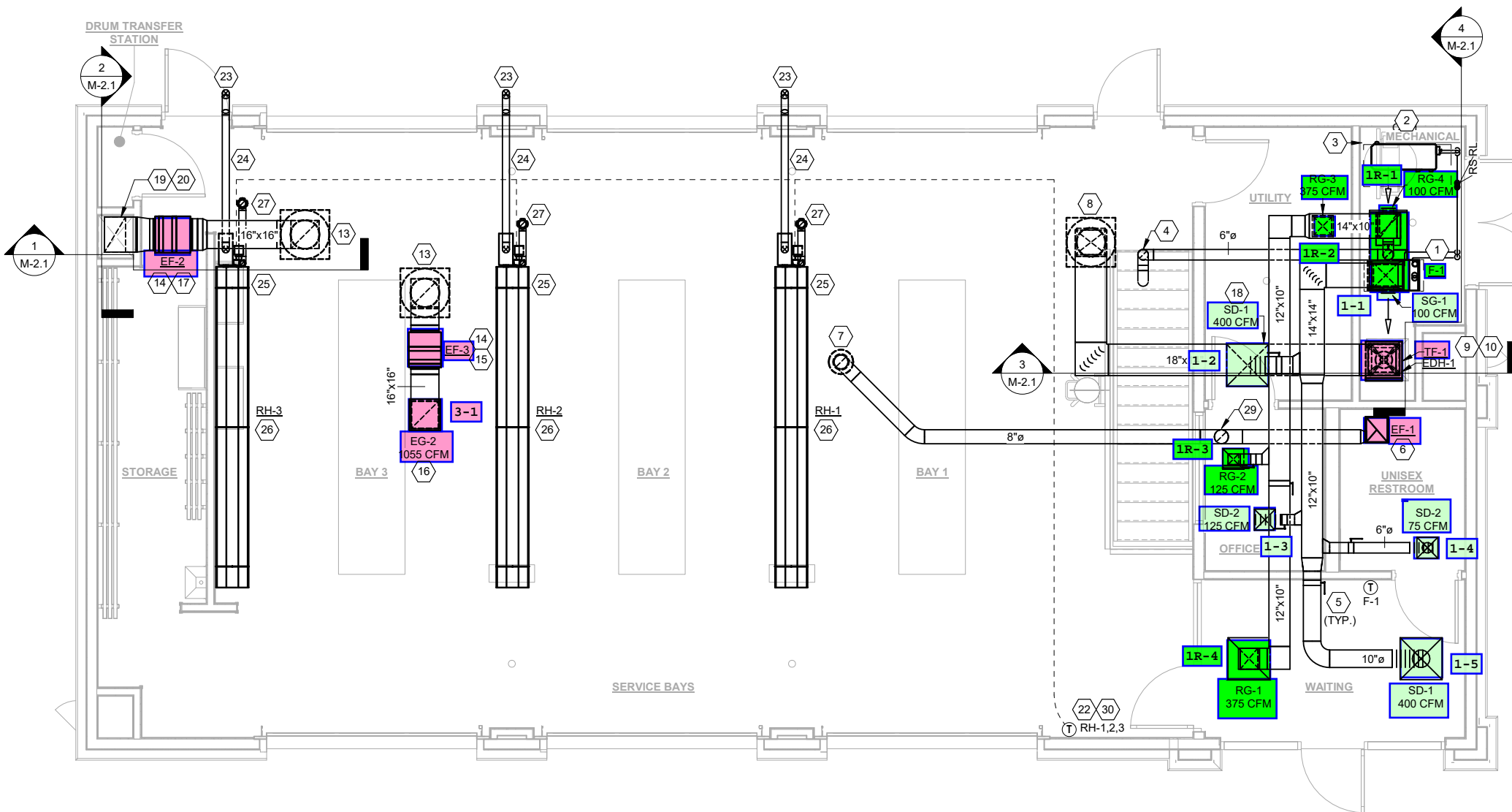
1 UPPER LEVEL MECHANICAL PLAN M-1.1 Scale: 1/4" = 1'-0"
