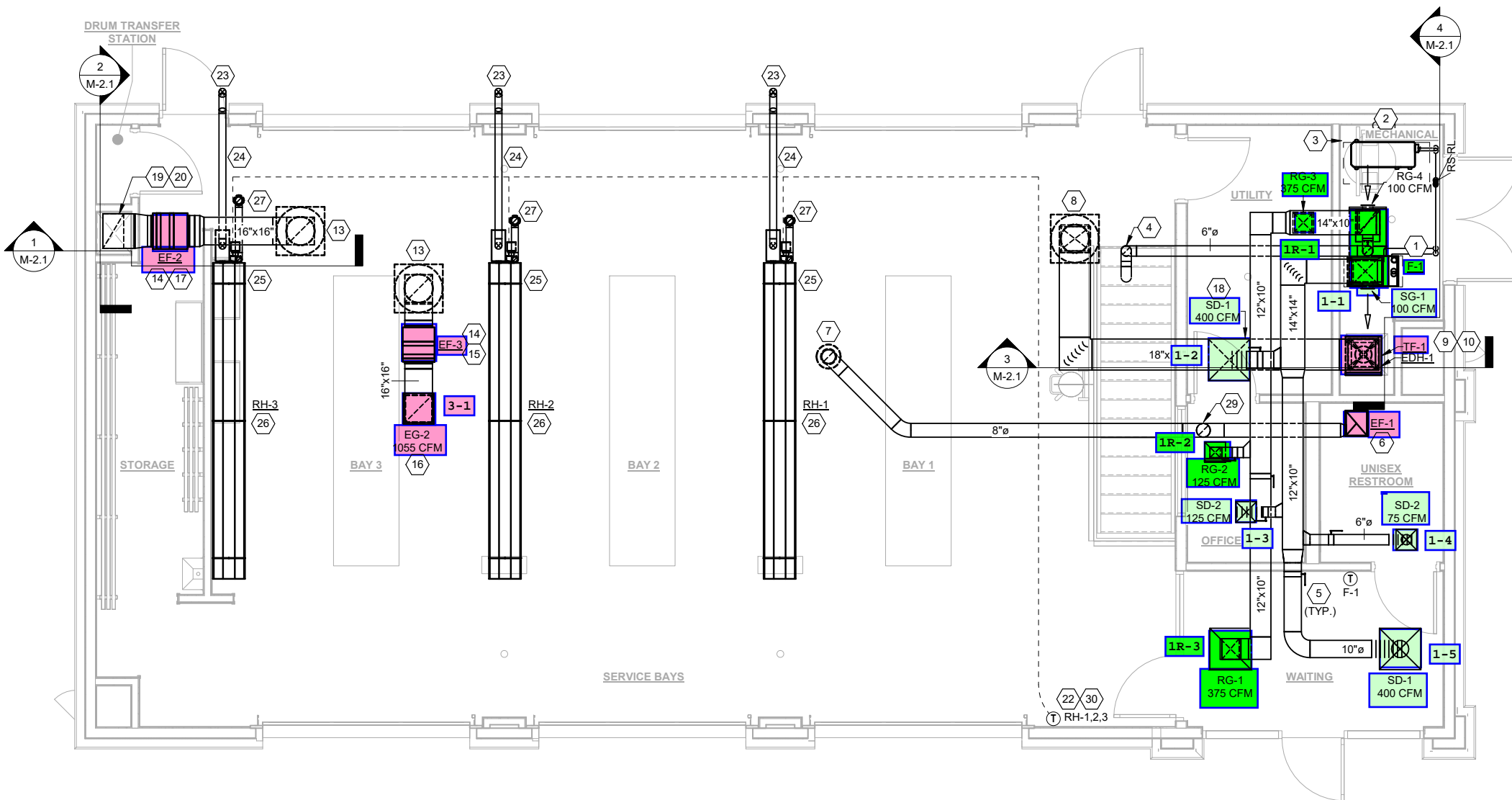
1 UPPER LEVEL MECHANICAL PLAN M-1.1 Scale: 1/4" = 1'-0"
