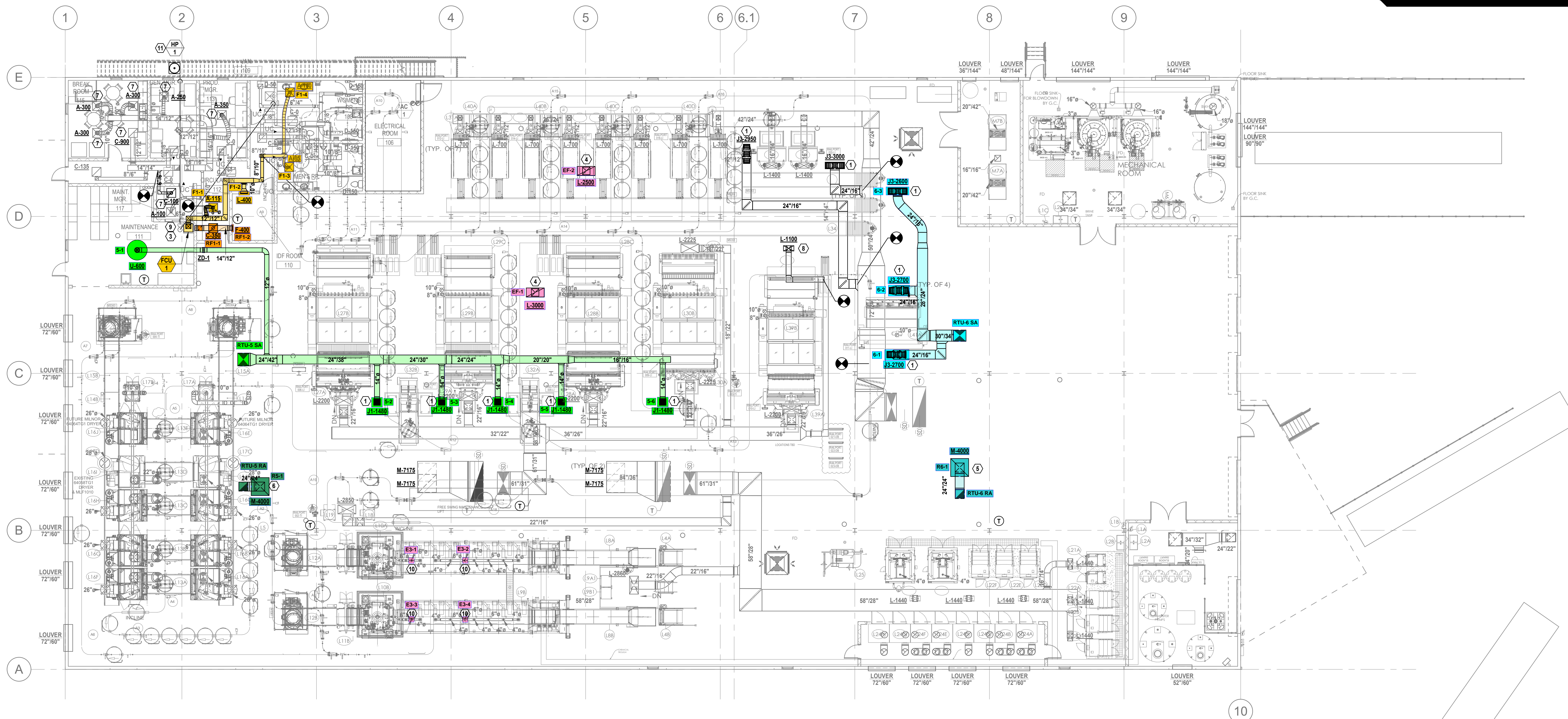
1 FLOOR PLAN - MECHANICAL 3/32" = 1'-0"
