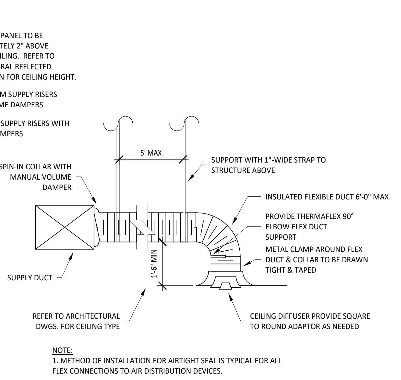
1 DIFFUSER CONNECTION N.T.S.
