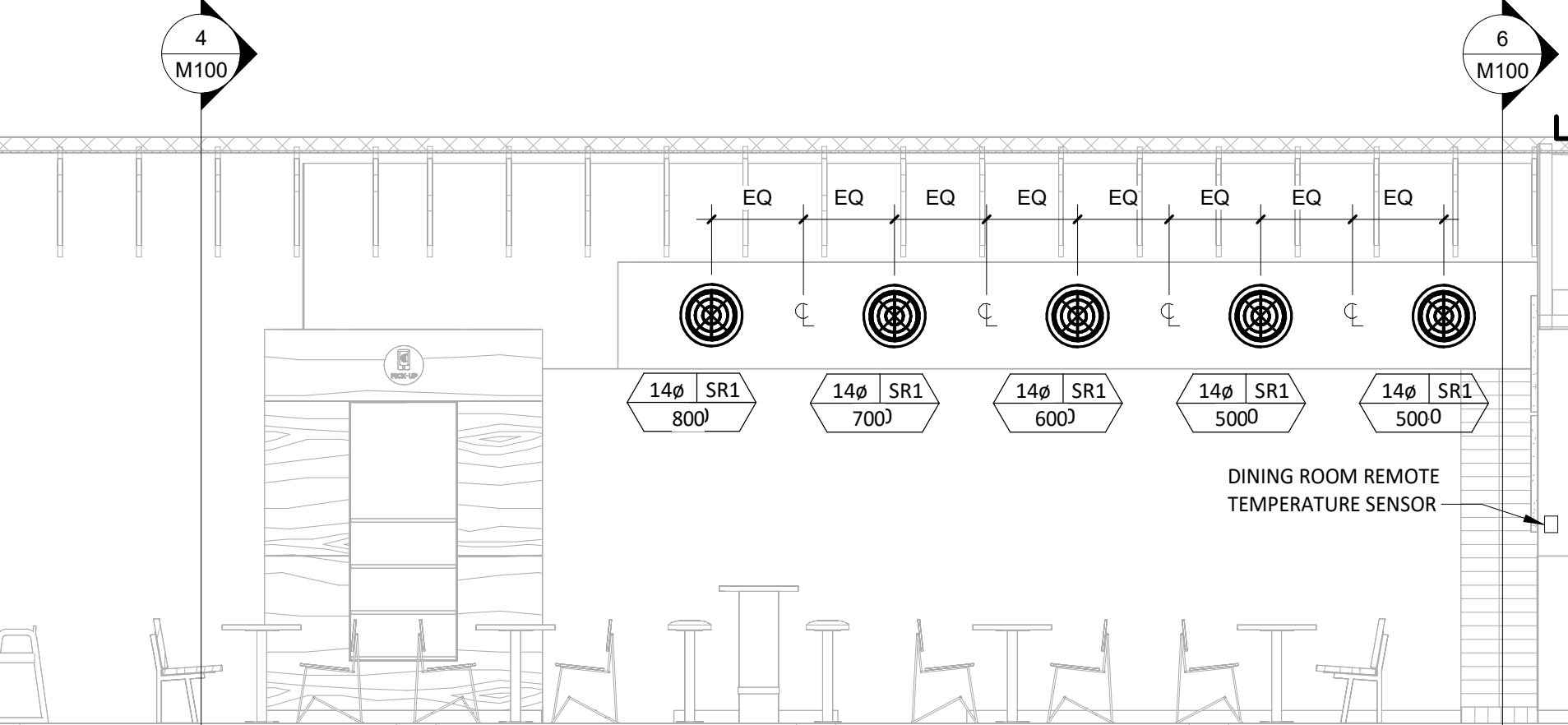
3 M100 HVAC DINING ROOM SECTION 1/4" = 1'-0"
