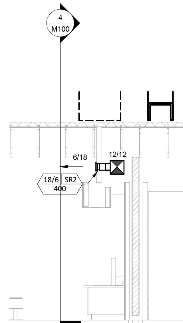
5 M100 HVAC DINING ROOM SECTION 1/4" = 1'-0"
