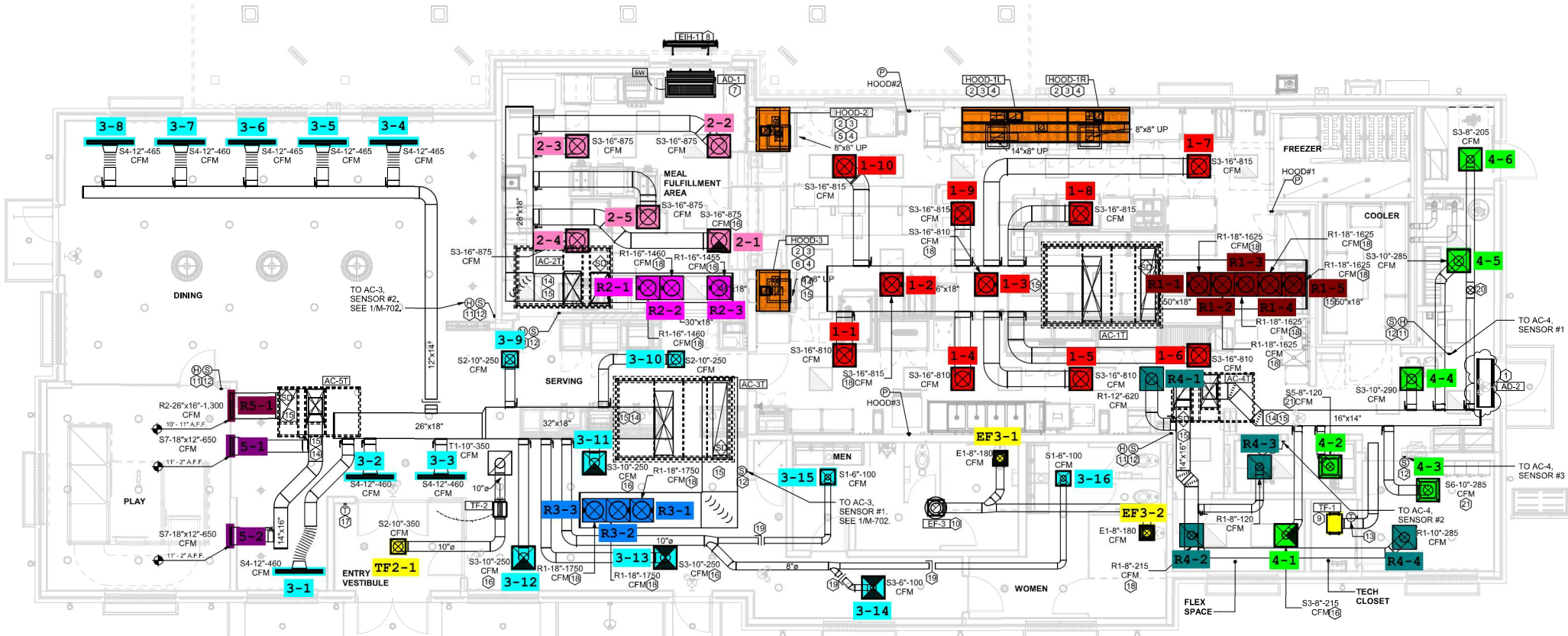
① EQUIPMENT AND DUCTWORK PLAN
