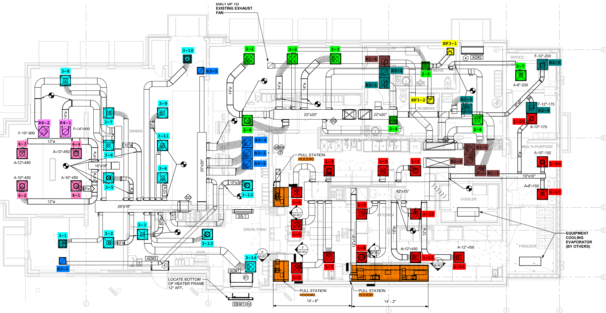
MECHANICAL FLOOR PLAN
