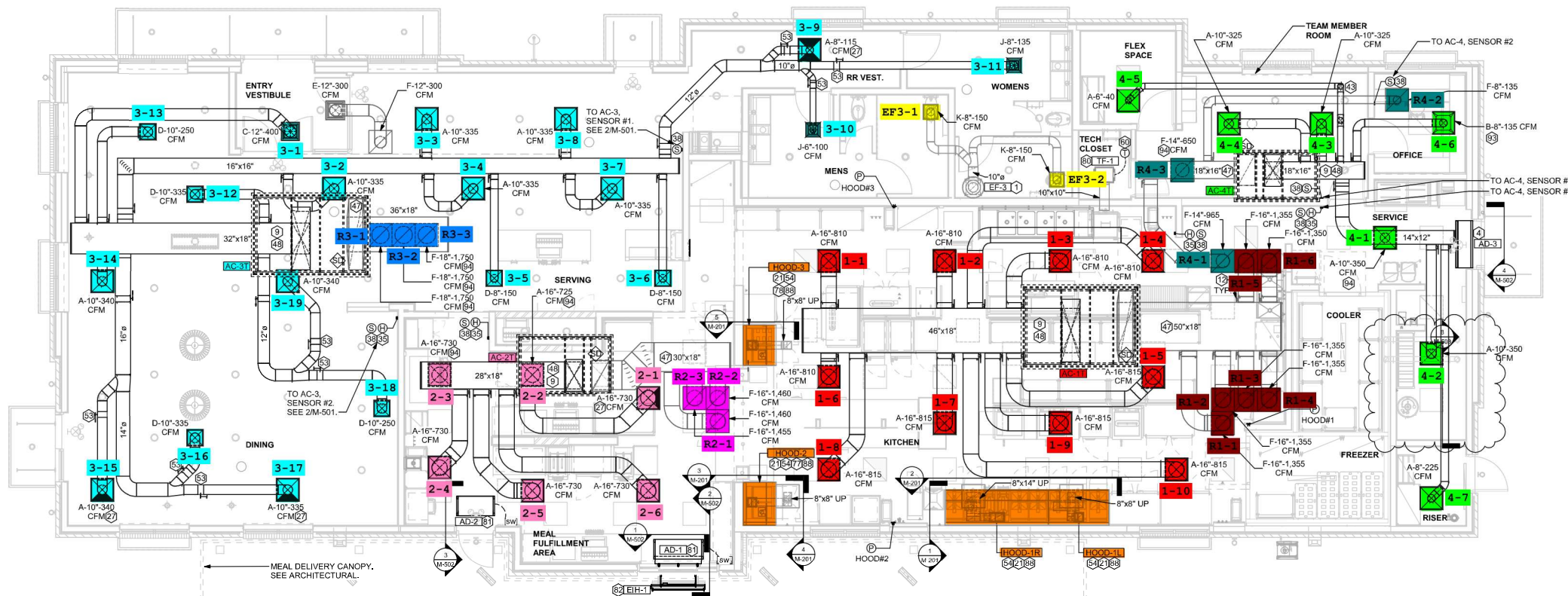
EQUIPMENT AND DUCTWORK PLAN
