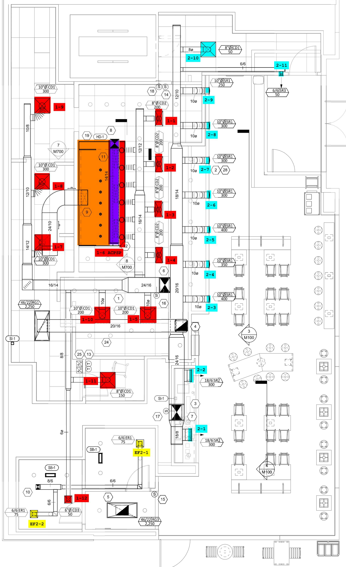
1 M100 HVAC FLOOR PLAN 1/4" = 1'-0"
