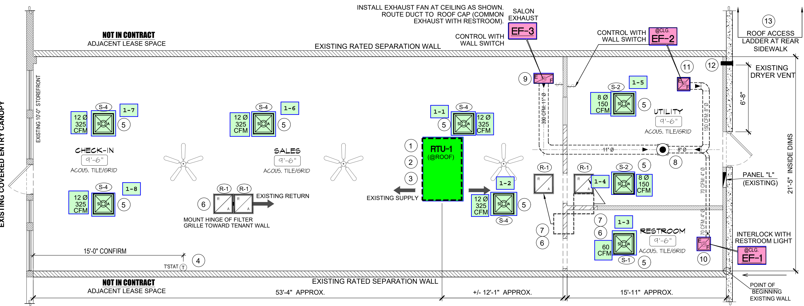
1 MECHANICAL PLAN - PROPOSED SCALE: 1/4"=1'-0"
