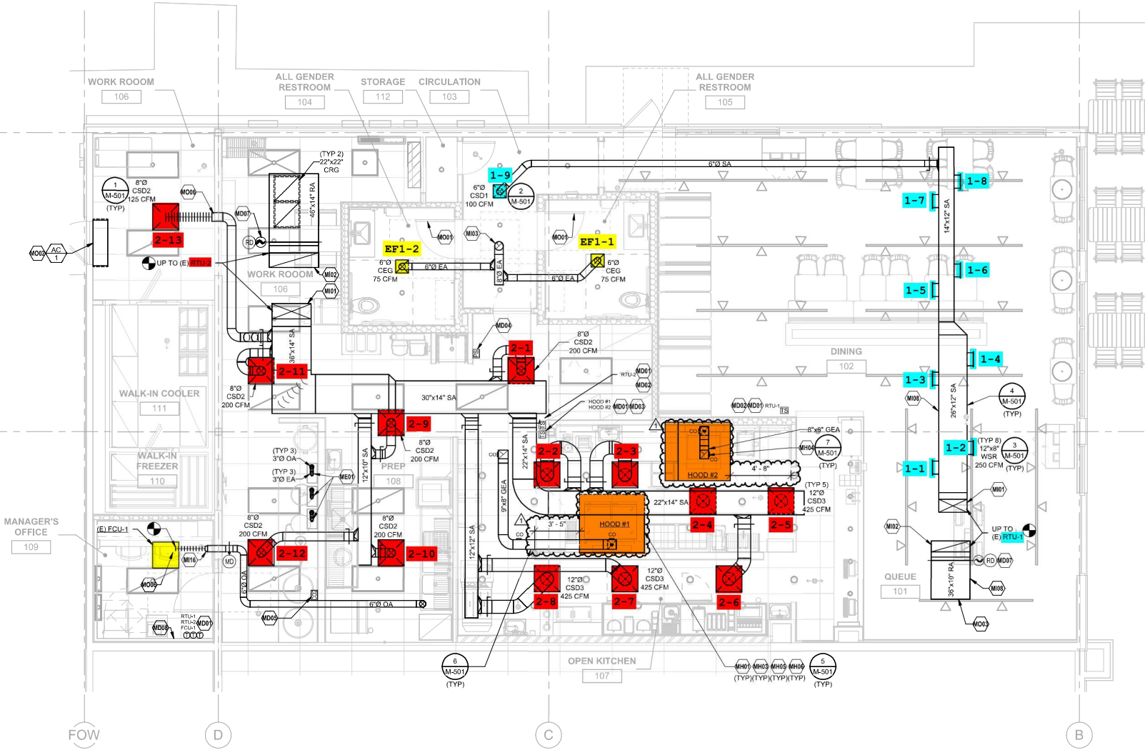
1 MECHANICAL FLOOR PLAN 1/4" = 1'-0"
