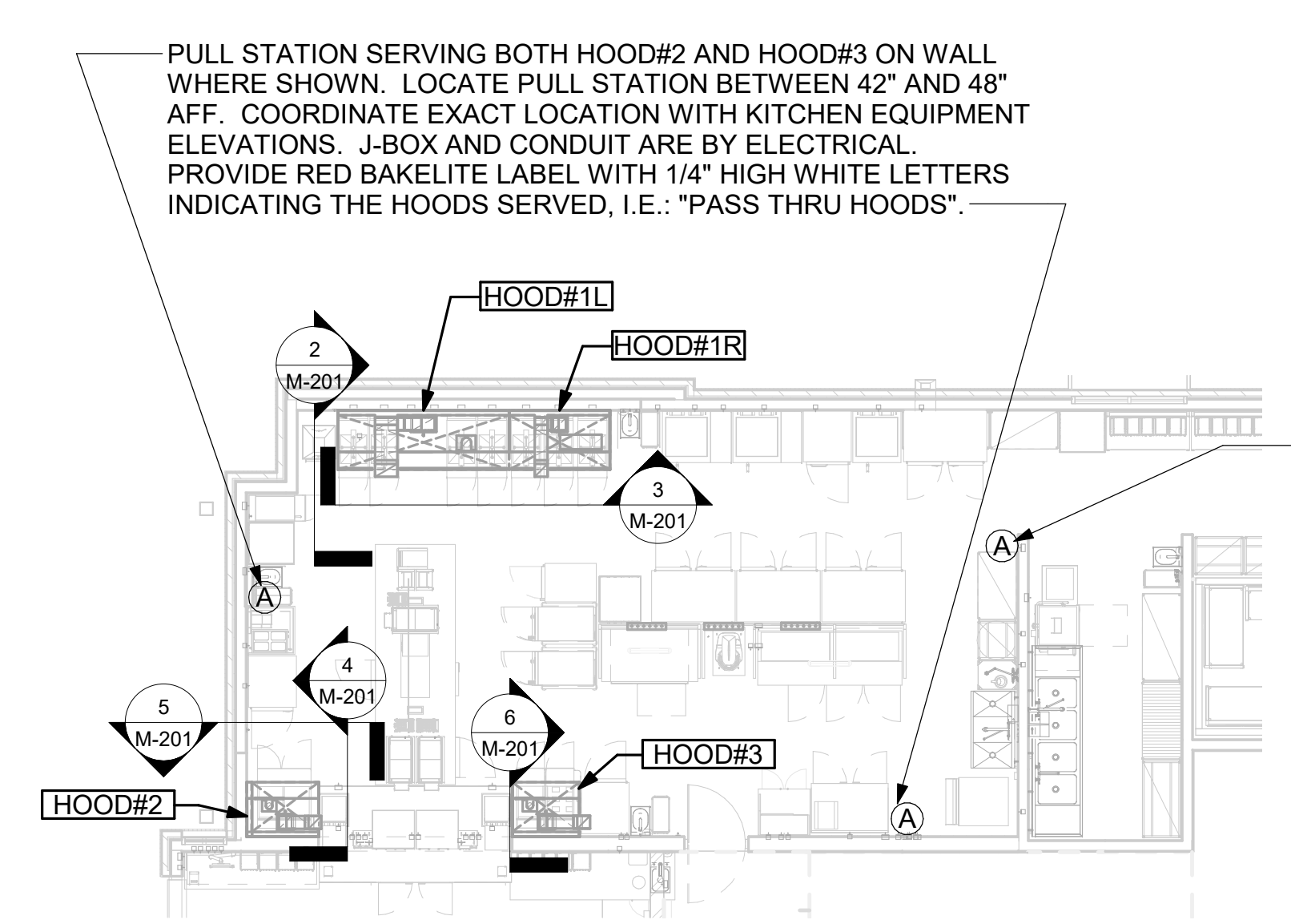
1 HOOD LAYOUT 1/8" = 1'-0"
