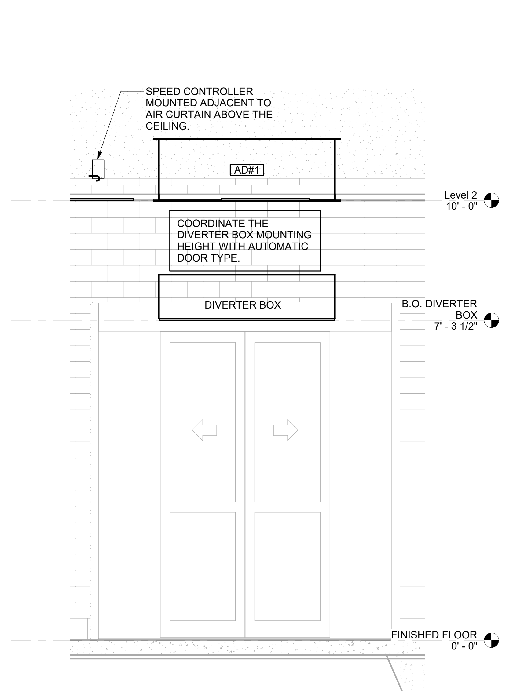
2 AD#1 FRONT VIEW 3/4" = 1'-0"
