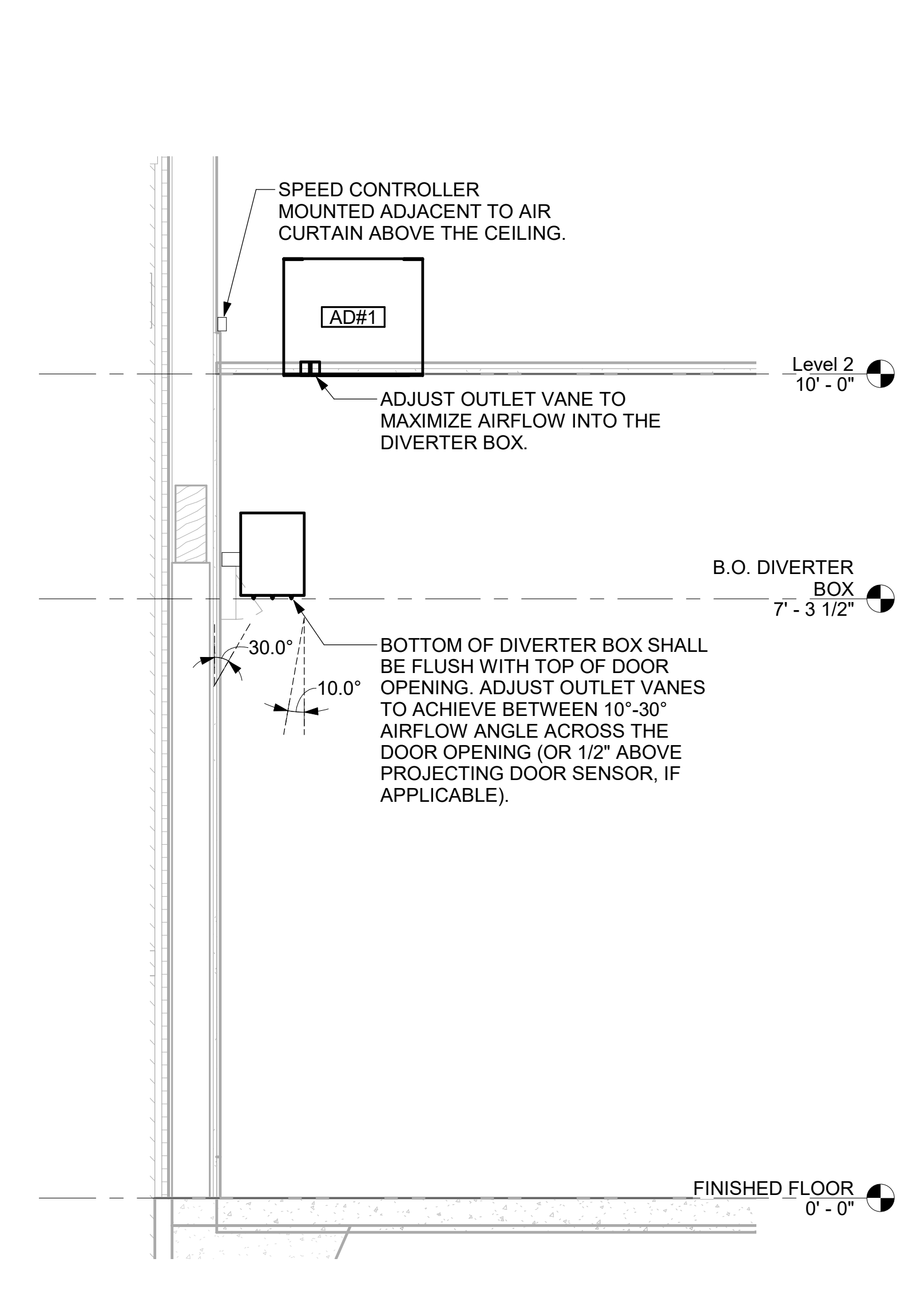
3 AD#1 SIDE VIEW 3/4" = 1'-0"
