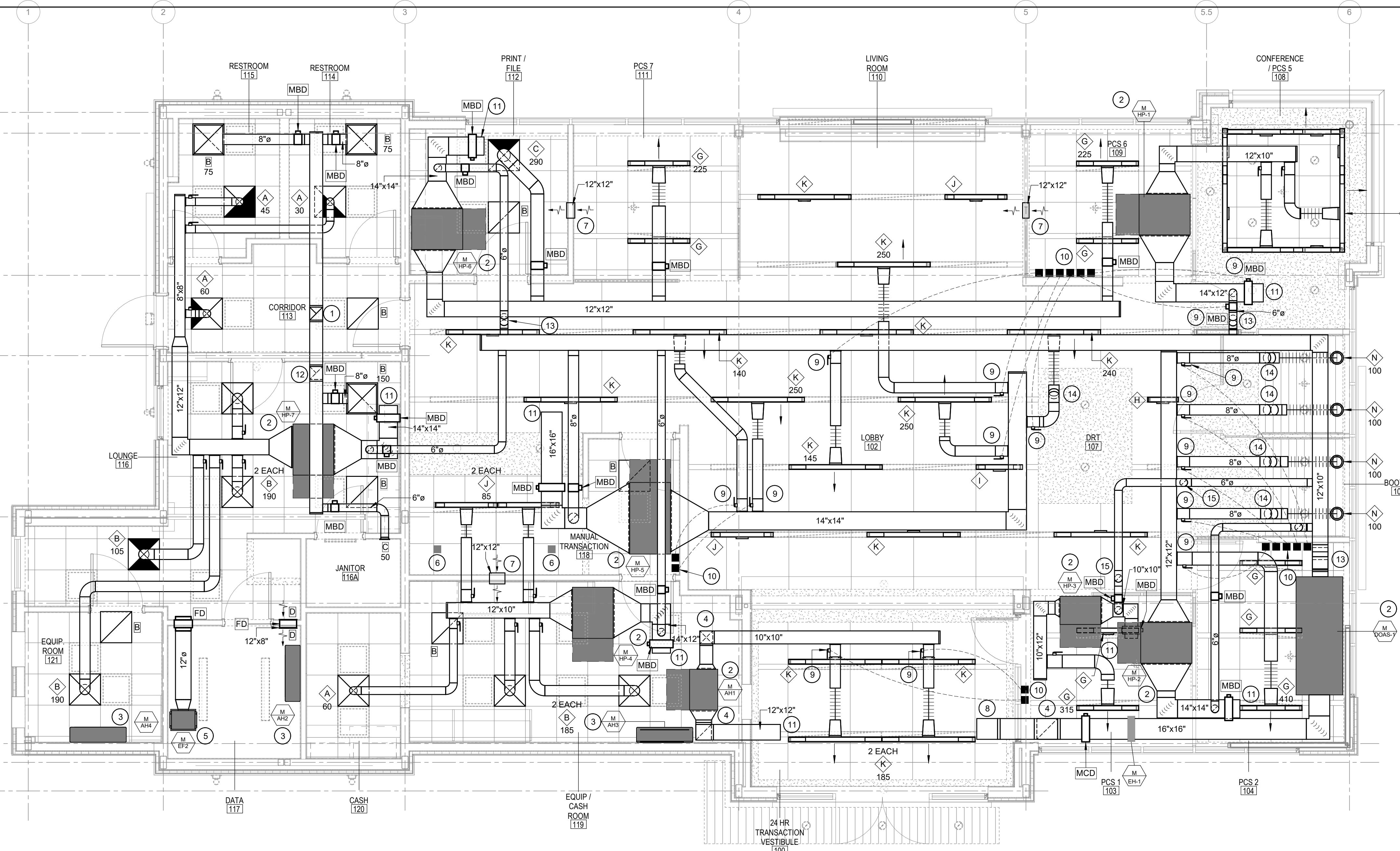
1 HVAC FLOOR PLAN M2.01 1/4" = 1'-0"
