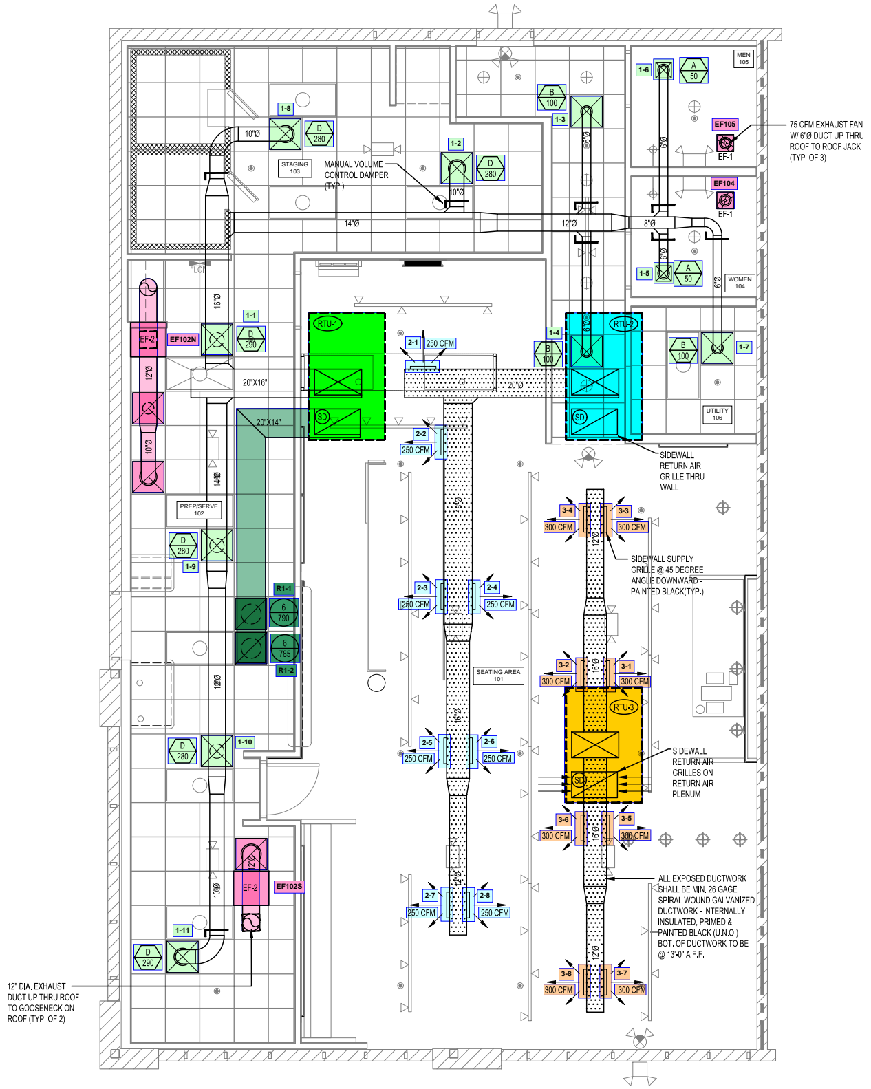
1 MECHANICAL PLAN
