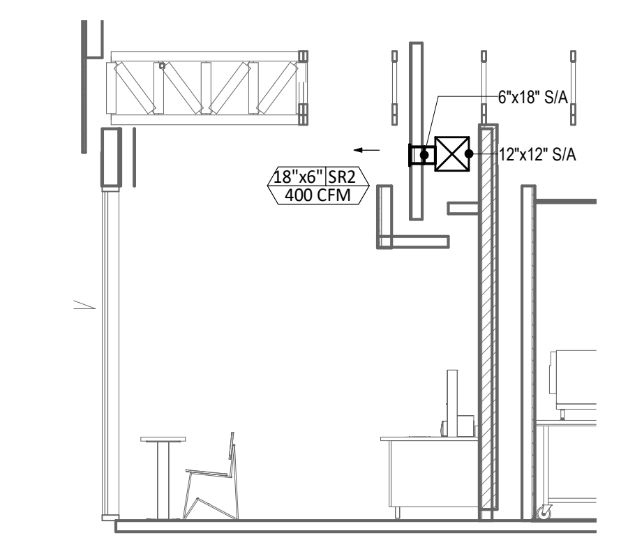
5 HVAC DINING ROOM SECTION 1/4" = 1'-0"
