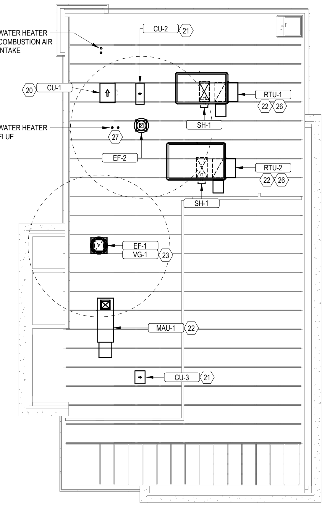
2 ROOF MECHANICAL PLAN 1/8" = 1'-0"
