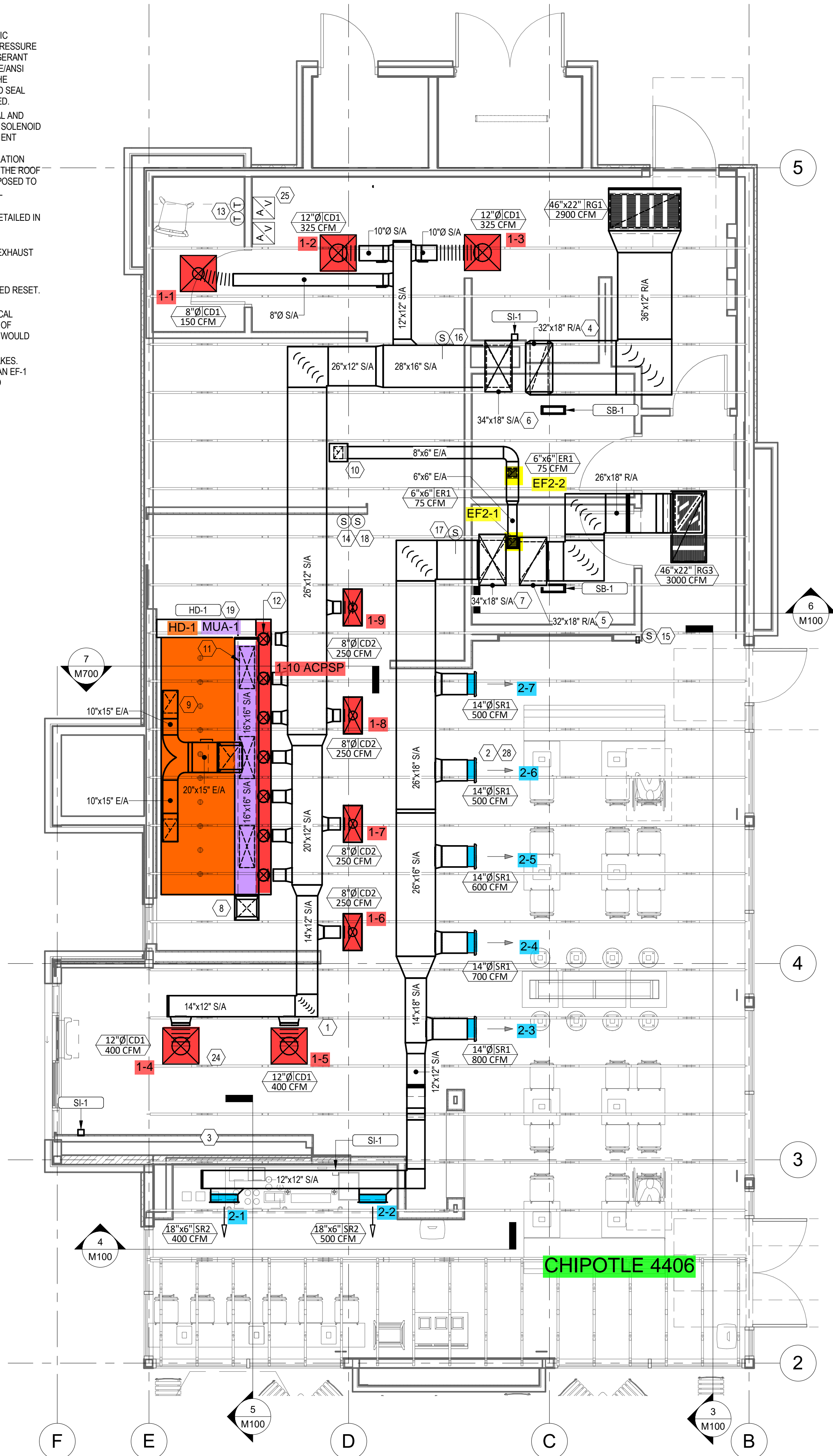
1 HVAC PLAN 1/4" = 1'-0"
