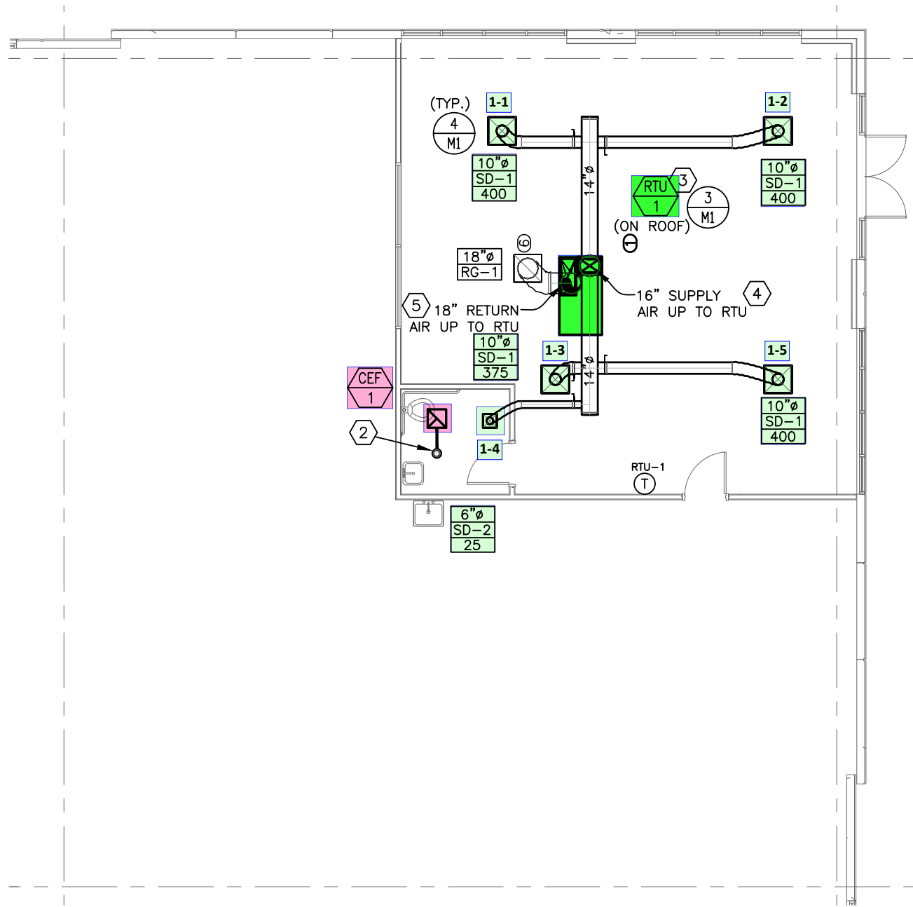
1 | Detail Mechanical Floor Plan
