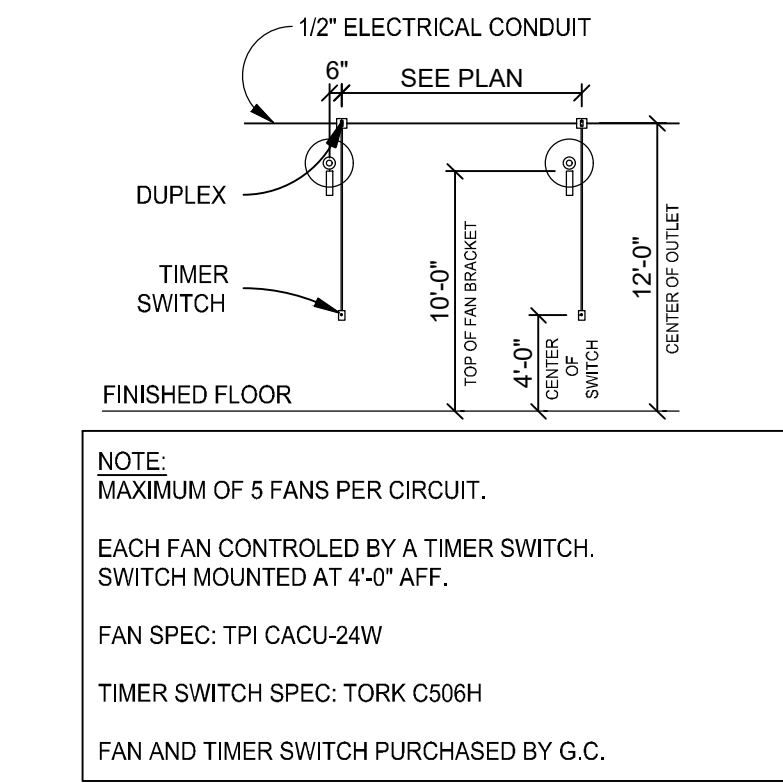
12 CIRCULATION FAN DETAILS SCALE: NONE
