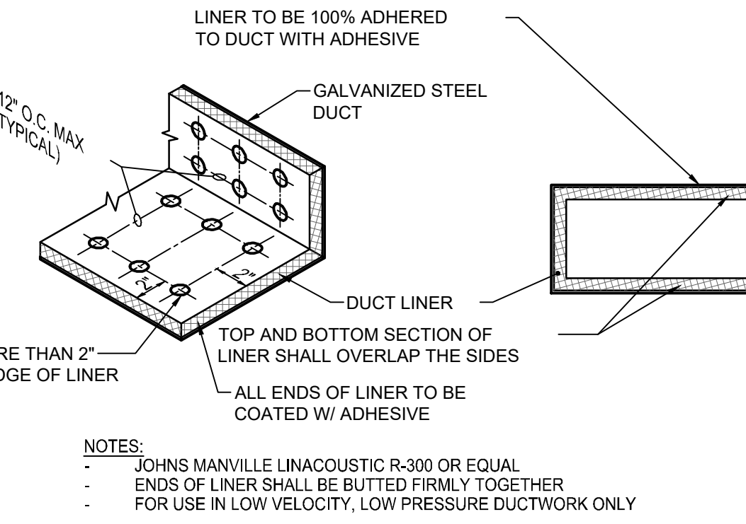
07 ACOUSTIC LINING DETAIL SCALE: NONE
