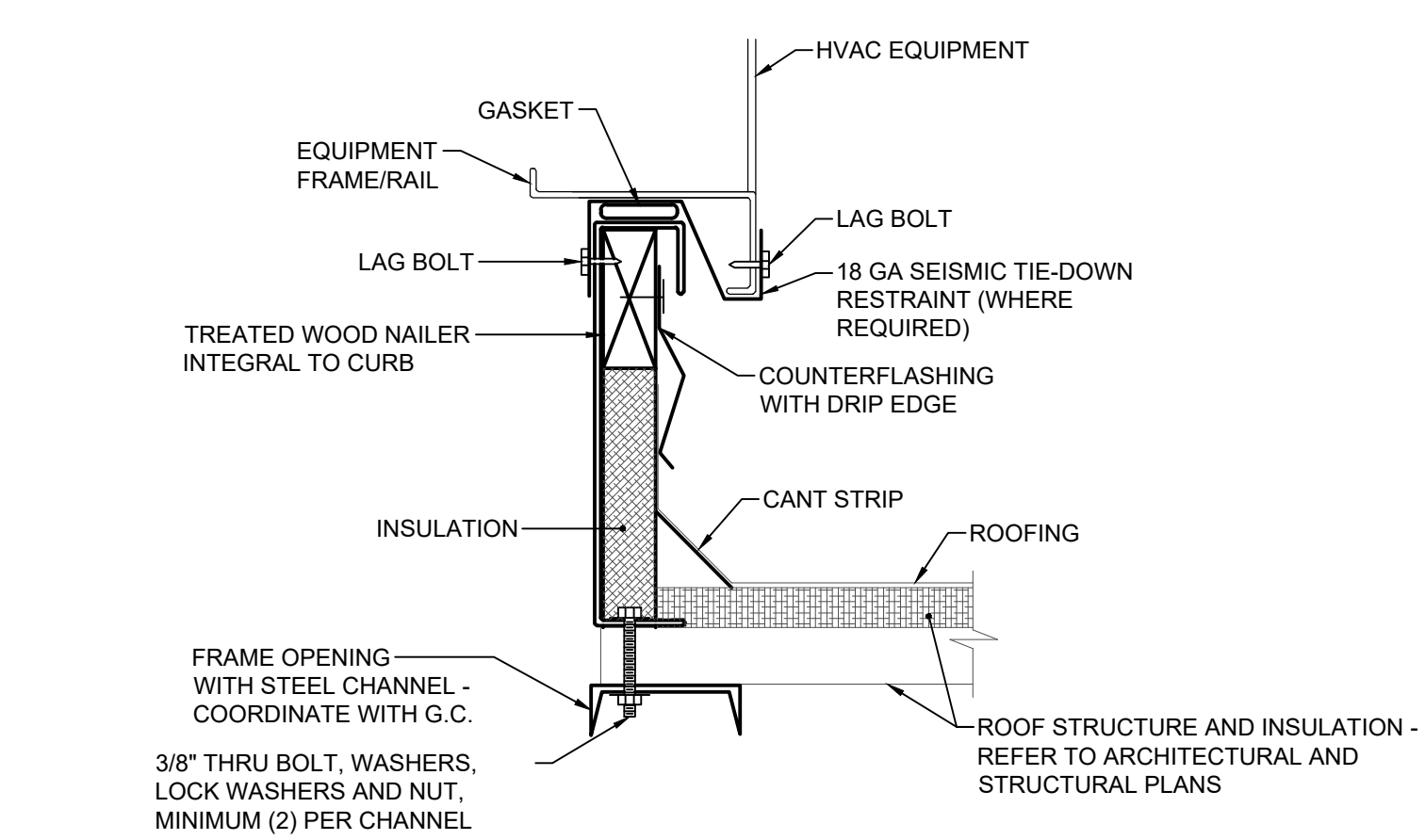
09 ROOFTOP UNIT CURB DETAIL SCALE: NONE
