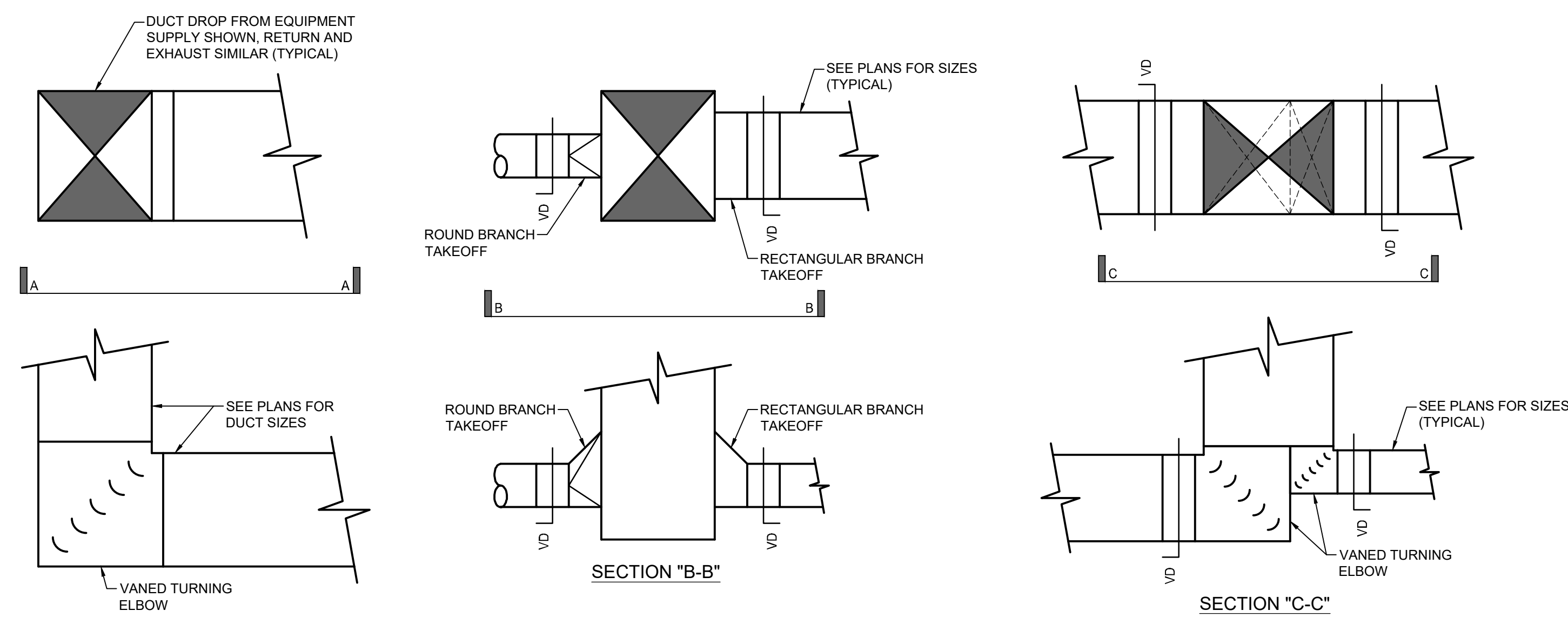
15 EQUIPMENT DUCT DROP DETAILS SCALE: NONE
