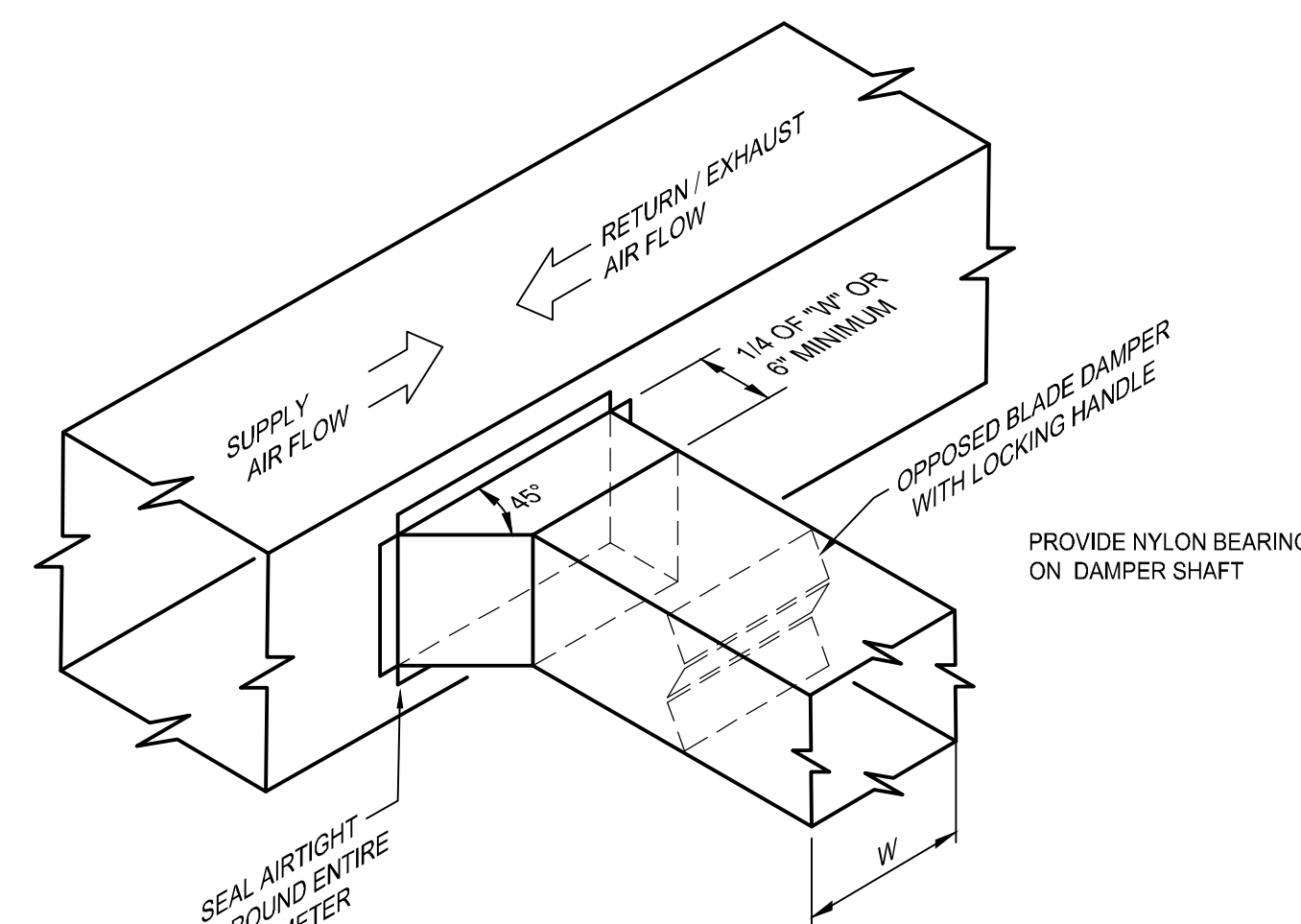
02 RECTANGULAR BRANCH TAKE-OFF SCALE: NONE
