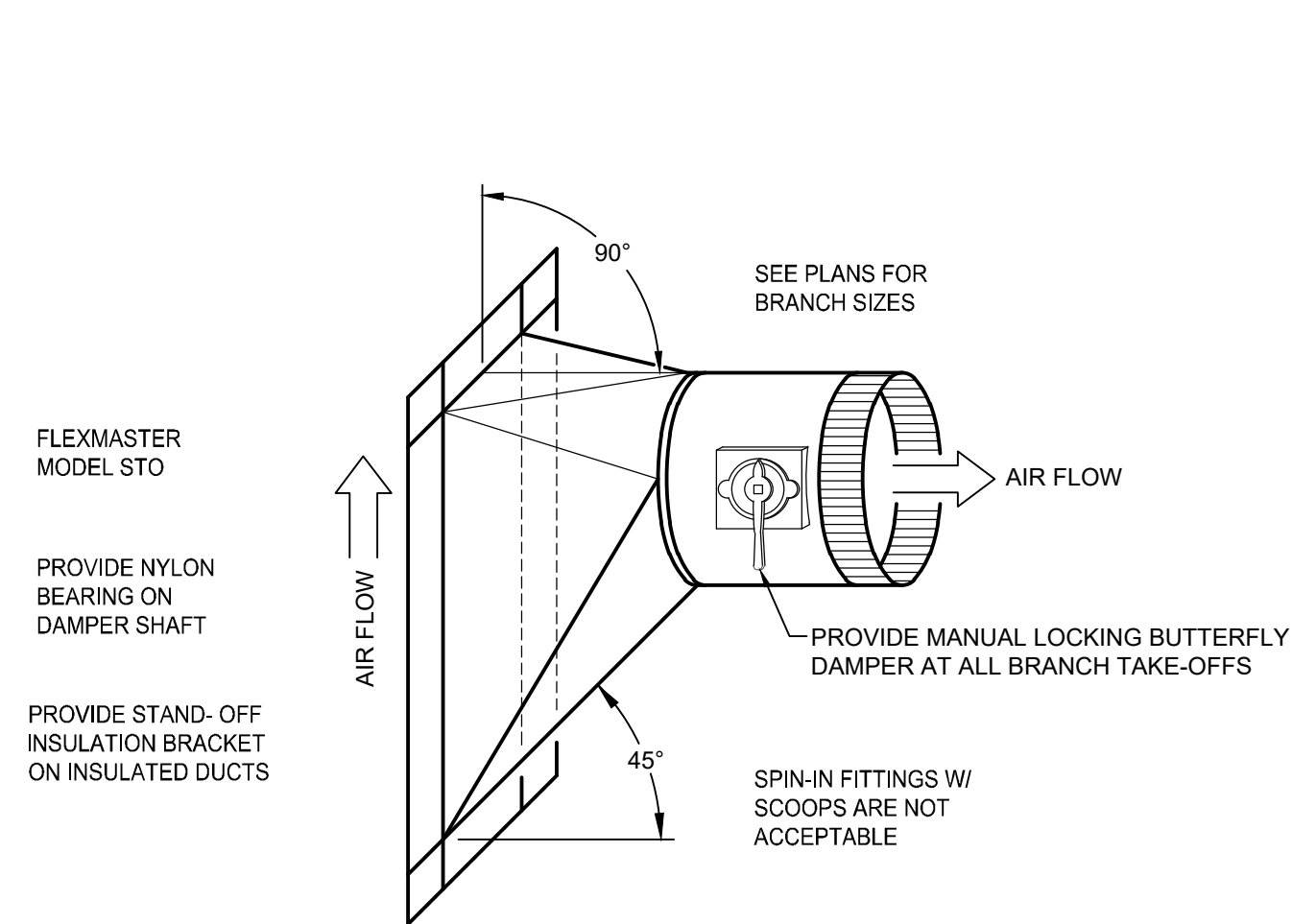
01 ROUND BRANCH TAKE-OFF SCALE: NONE
