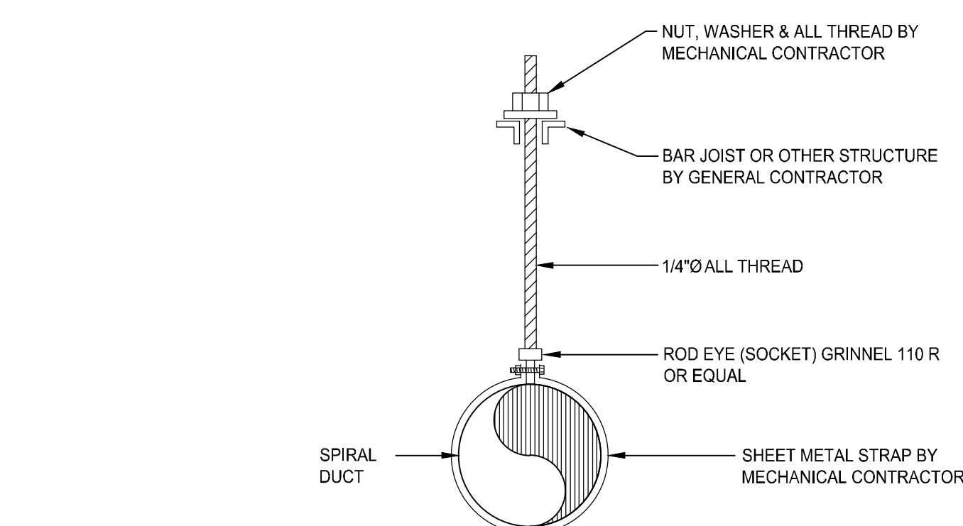
04 SPIRAL DUCT HANGER DETAIL SCALE: NONE
