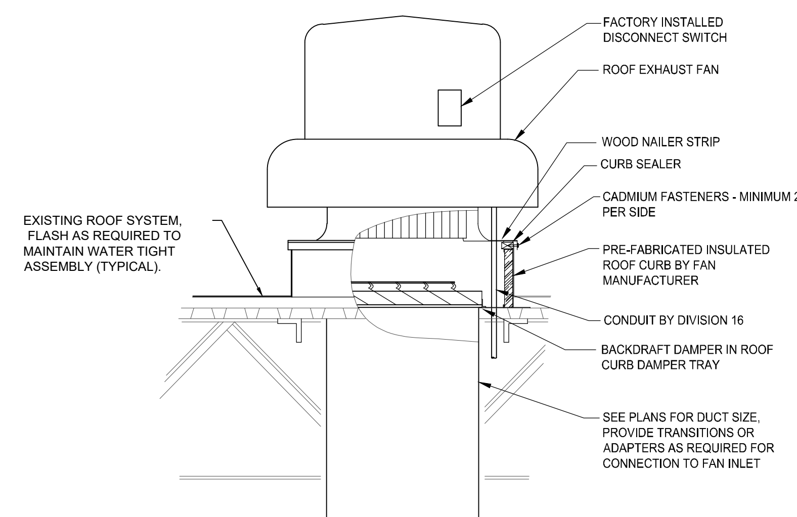
05 ROOF MOUNTED EXHAUST FAN DETAIL SCALE: NONE
