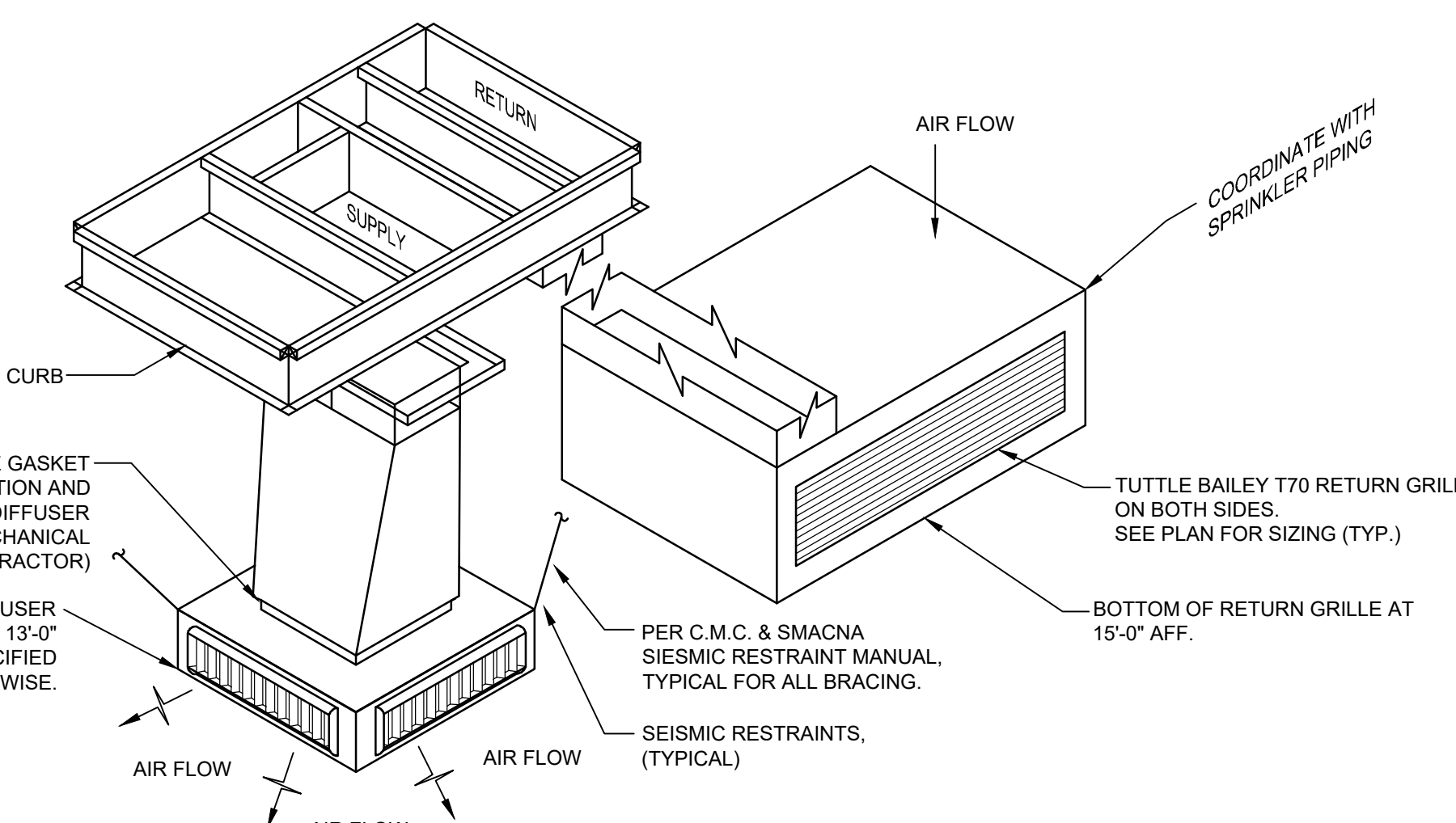
03 DRUM LOUVER DIFFUSER SCALE: NONE
