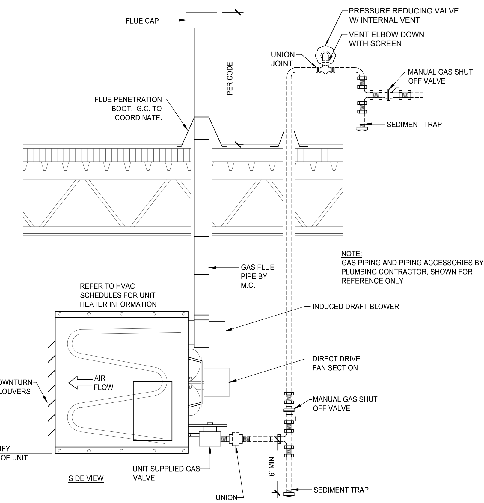
08 UNIT HEATER INSTALLATION DETAIL SCALE: NONE
