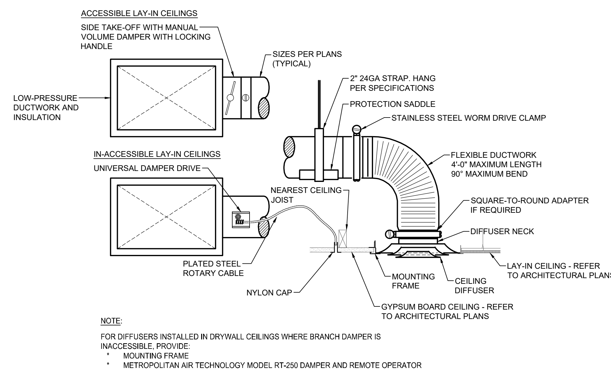
10 CEILING DIFFUSER DETAIL SCALE: NONE
