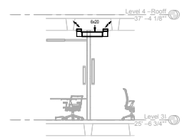
2 TYPICAL TRANSFER AIR DUCT SCALE: 1/4" = 1'-0"
