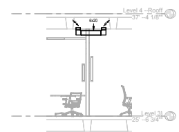
2 TYPICAL TRANSFER AIR DUCT SCALE: 1/8" = 1'-0"
