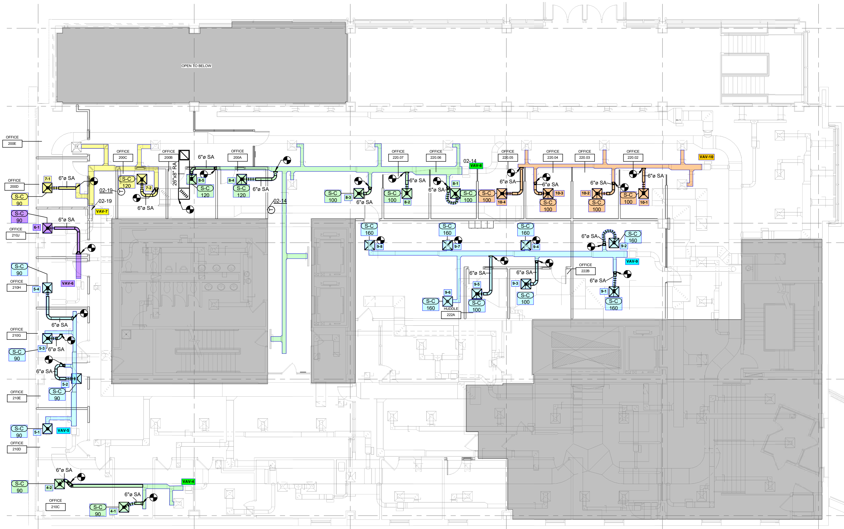
1 MECHANICAL PLAN - LEVEL 200
