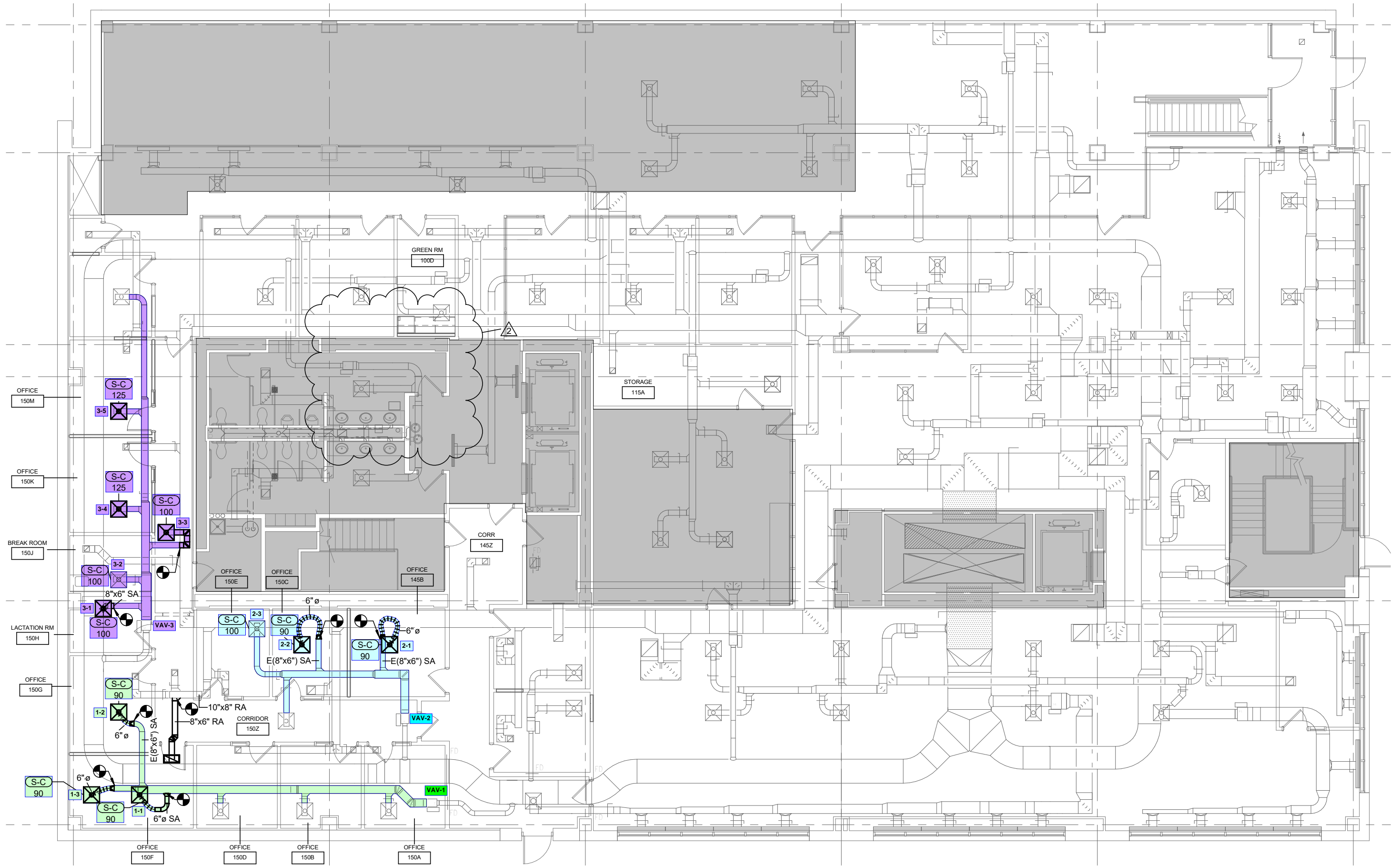
1 MECHANICAL PLAN - LEVEL 100
